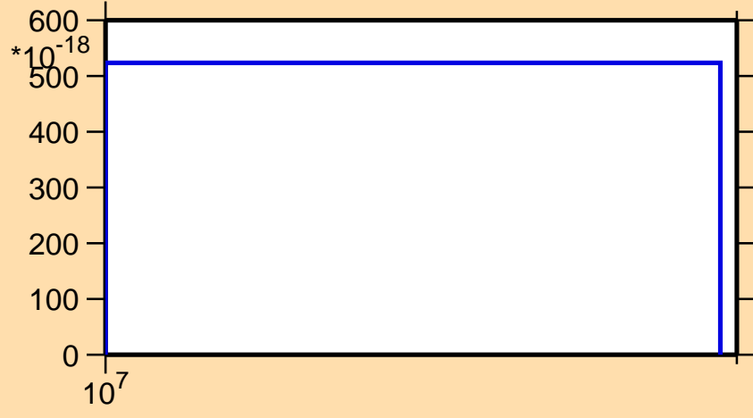
\sigma vs. E for ^{113}\text{Sn} (mt 45)
