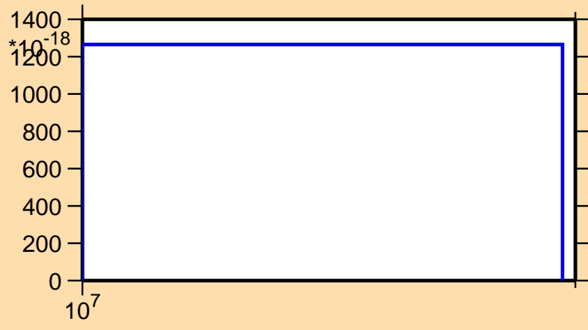
\sigma vs. E for ^{113}\text{Sn}(\text{mt117})
