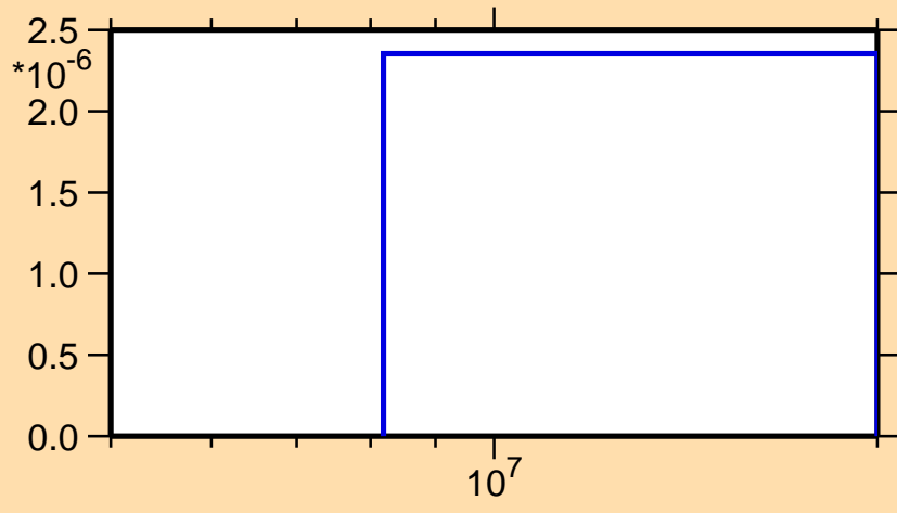
\sigma vs. E for ^{113}\text{Sn}(n,3n)
