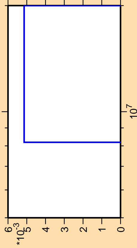
\Delta\sigma/\sigma vs. E for ^{113}\text{Sn}(\text{mt } 45)
