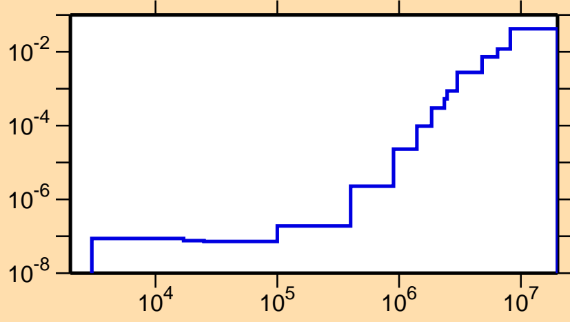
\sigma vs. E for ^{113}\text{Sn}(n,p)
