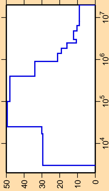
\Delta\sigma/\sigma vs. E for ^{113}\text{Sn}(n,\text{nonel.})
