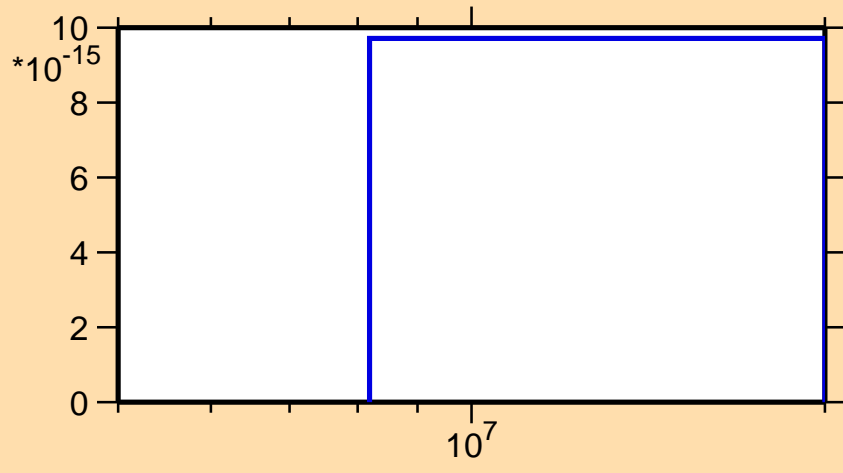
\sigma vs. E for ^{113}\text{Sn}(n,nt)
