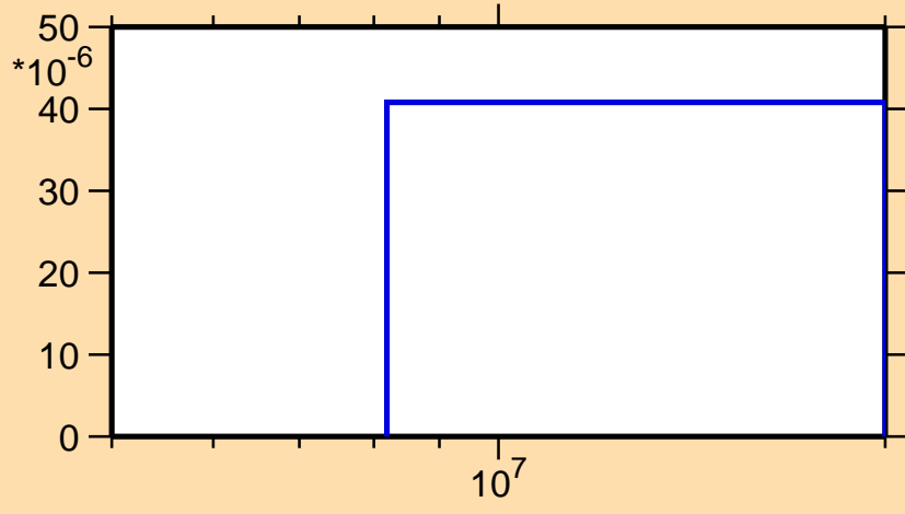
\sigma vs. E for ^{113}\text{Sn}(n,t)
