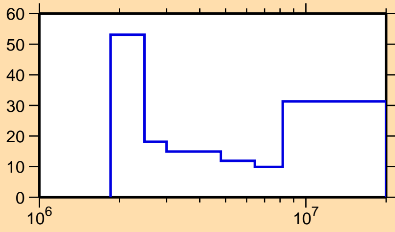
\Delta\sigma/\sigma vs. E for ^{113}\text{Sn}(n,n\text{cont.})
