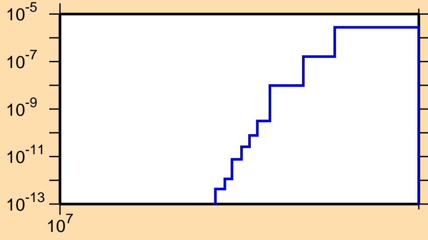
\sigma vs. E for ^{113}\text{Sn}(n,2n\alpha)
