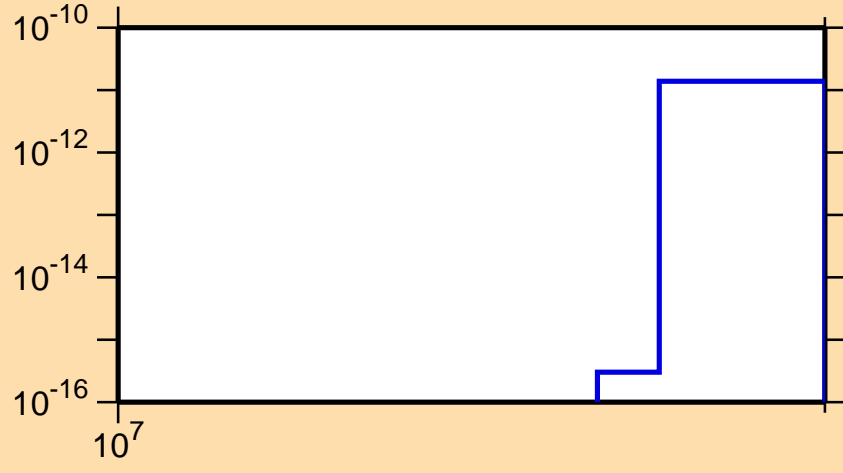
\sigma vs. E for ^{113}\text{Sn}(n,\text{pt})
