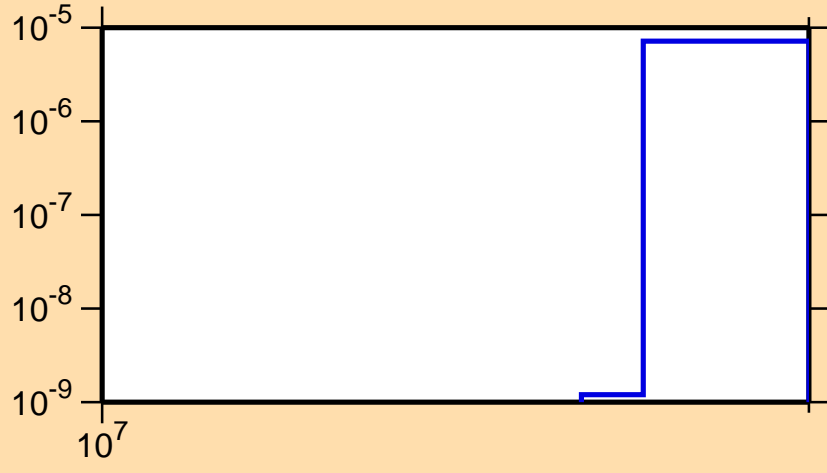
\sigma vs. E for ^{113}\text{Sn}(n,2np)
