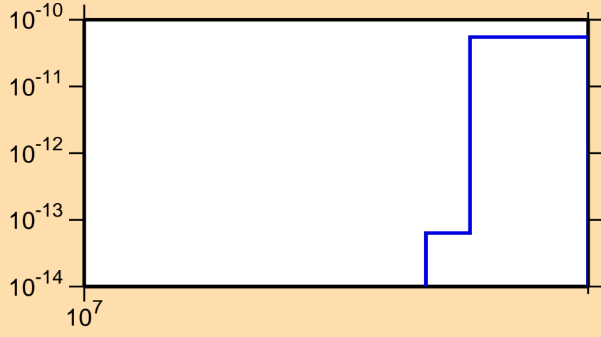
\sigma vs. E for ^{113}\text{Sn}(n,\text{pd})
