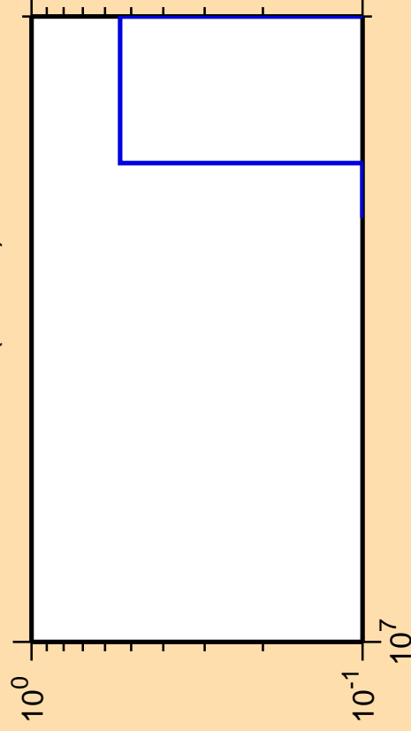
\Delta\sigma/\sigma vs. E for ^{113}\text{Sn}(\text{mt } 45)
