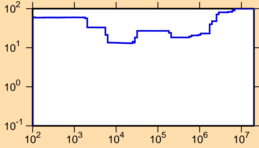
\Delta\sigma/\sigma vs. E for ^{113}\text{Sn}(n,\gamma)
