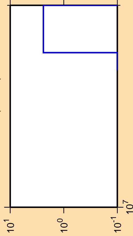
\Delta\sigma/\sigma vs. E for ^{113}\text{Sn}(\text{mt } 34)
