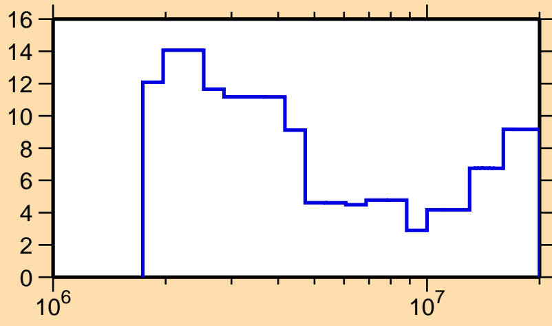
\Delta\sigma/\sigma vs. E for ^{113}\text{Sn}(n,\text{tot.})
