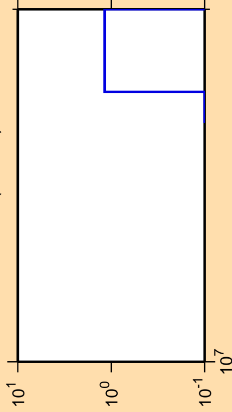
\Delta\sigma/\sigma vs. E for ^{113}\text{Sn}(\text{mt117})
