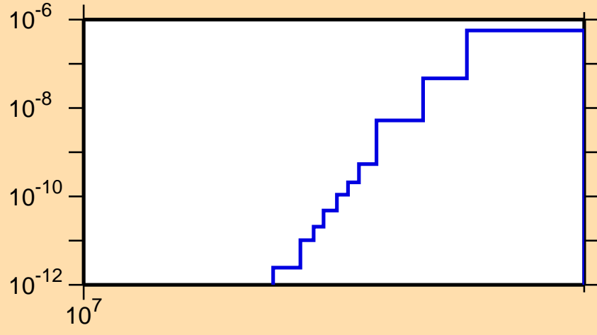
\sigma vs. E for ^{113}\text{Sn}(n,\text{He3})
