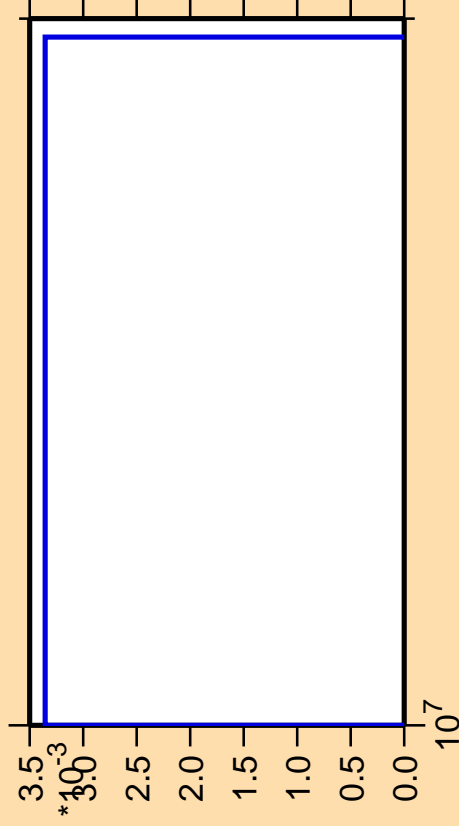
\Delta\sigma/\sigma vs. E for ^{113}\text{Sn} (mt 45)
