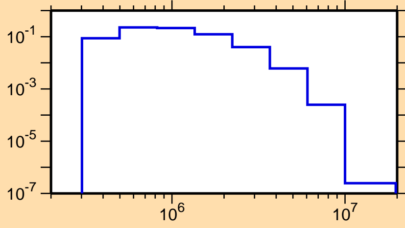
\sigma vs. E for ^{113}\text{Sn}(n,n_2)
