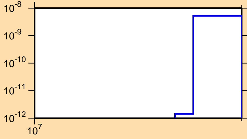
\sigma vs. E for ^{114}\text{Sn}(n,\text{nd})
