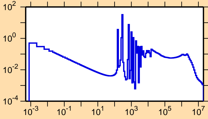
\sigma vs. E for ^{114}\text{Sn}(n,\gamma)
