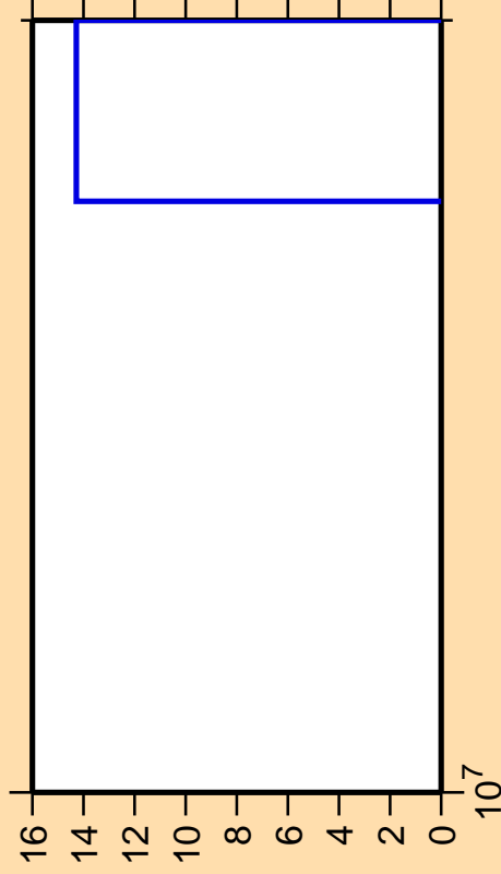
\Delta\sigma/\sigma vs. E for ^{114}\text{Sn}(n,2np)
