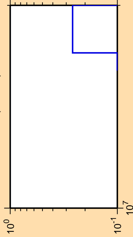
\Delta\sigma/\sigma vs. E for ^{114}\text{Sn}(\text{mt117})
