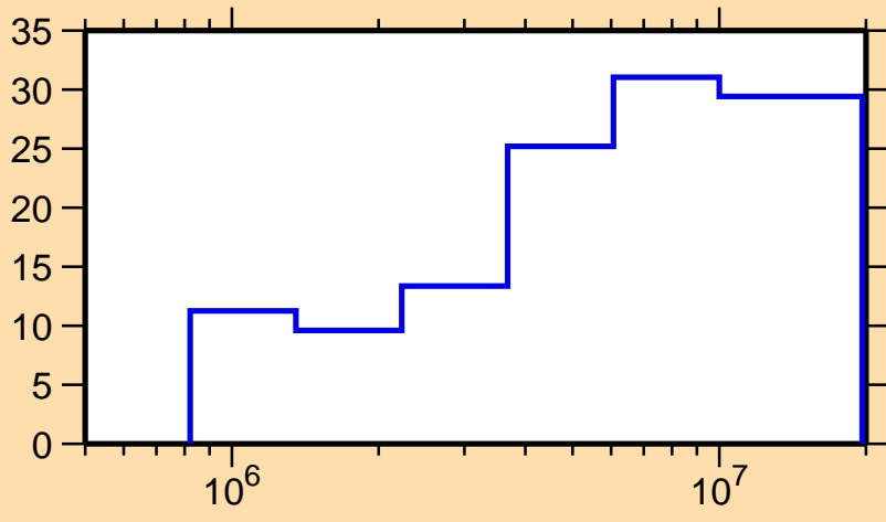
\Delta\sigma/\sigma vs. E for ^{114}\text{Sn}(n,n_1)
