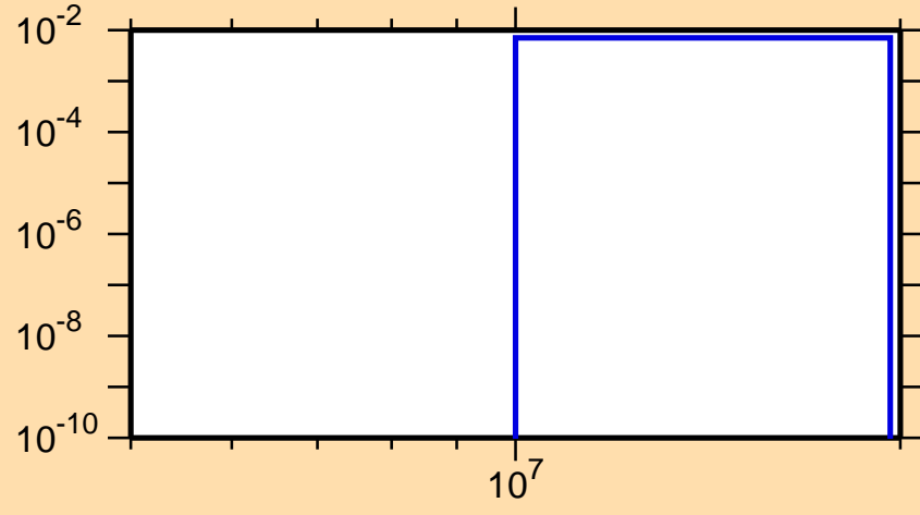
\sigma vs. E for ^{114}\text{Sn}(n,np)
