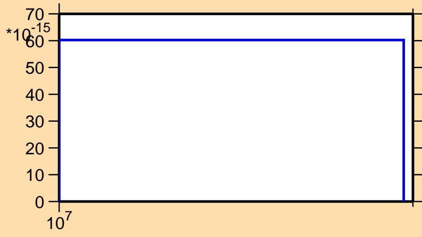
\sigma vs. E for ^{114}\text{Sn}(n,2np)
