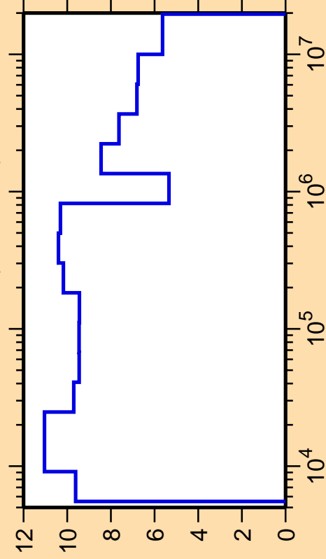
\Delta\sigma/\sigma vs. E for ^{114}\text{Sn}(n,\text{nonel.})
