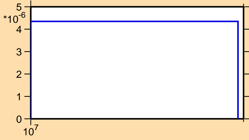
\sigma vs. E for ^{114}\text{Sn}(n,t)
