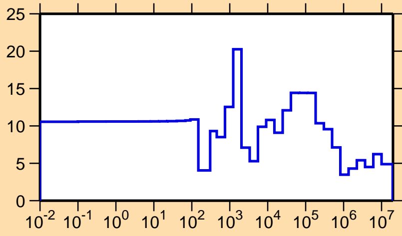
\Delta\sigma/\sigma vs. E for ^{114}\text{Sn}(n,\text{el.})
