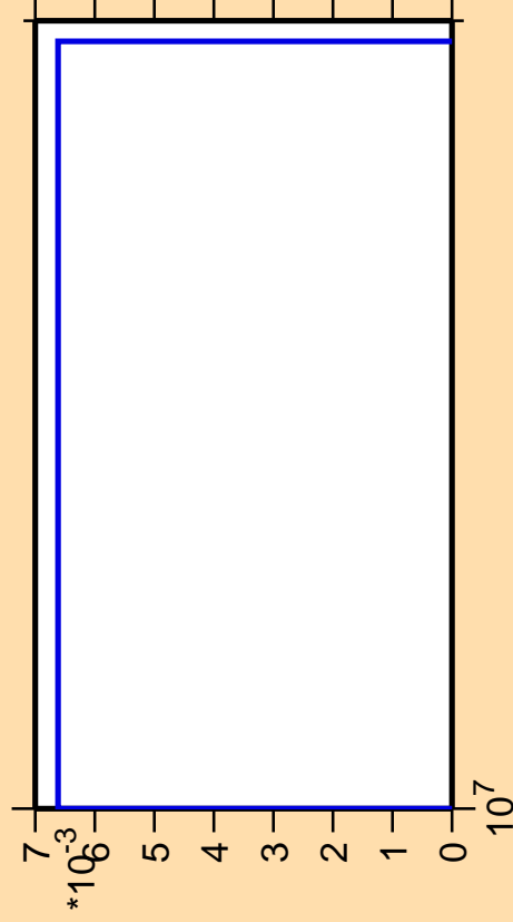
\Delta\sigma/\sigma vs. E for ^{114}\text{Sn}(n,nt)
