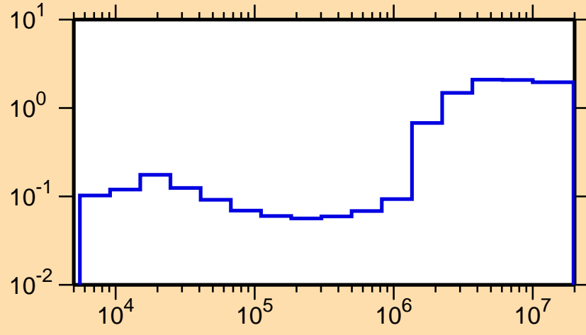
\sigma vs. E for ^{114}\text{Sn}(n,\text{nonel.})
