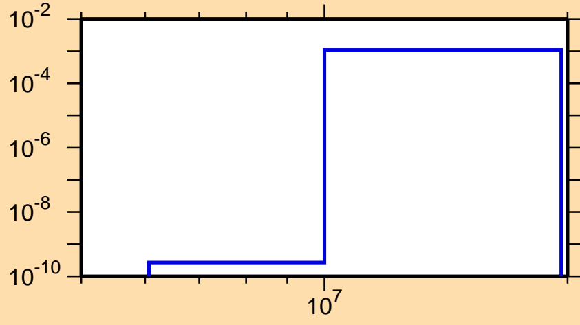
\sigma vs. E for ^{114}\text{Sn}(n,d)
