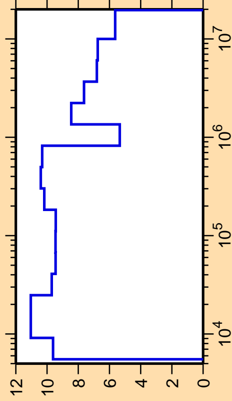
\Delta\sigma/\sigma vs. E for ^{114}\text{Sn}(n,\text{nonel.})
