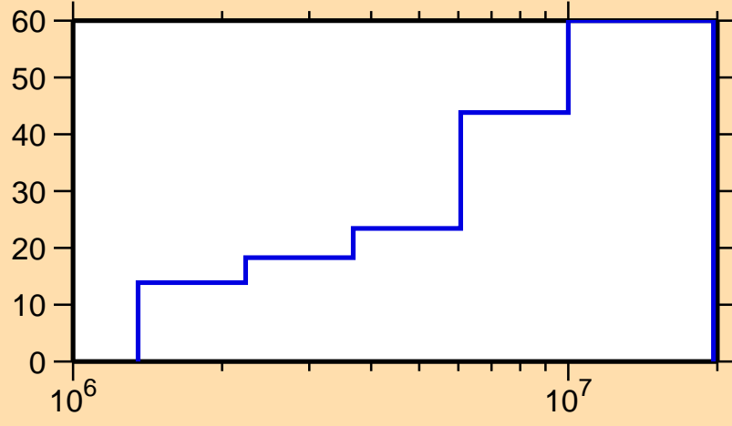
\Delta\sigma/\sigma vs. E for ^{114}\text{Sn}(n,\gamma)
