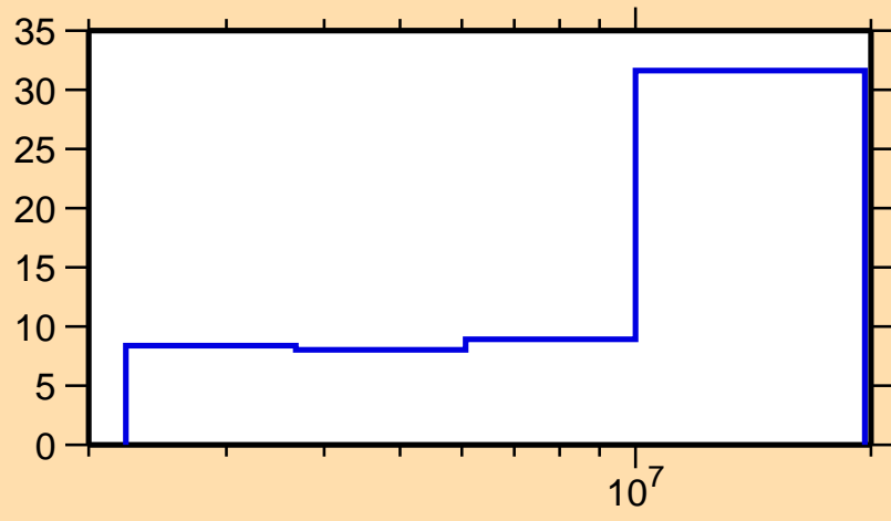
\Delta\sigma/\sigma vs. E for ^{114}\text{Sn}(n,n\text{cont.})
