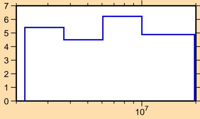
\Delta\sigma/\sigma vs. E for ^{114}\text{Sn}(n,\text{el.})
