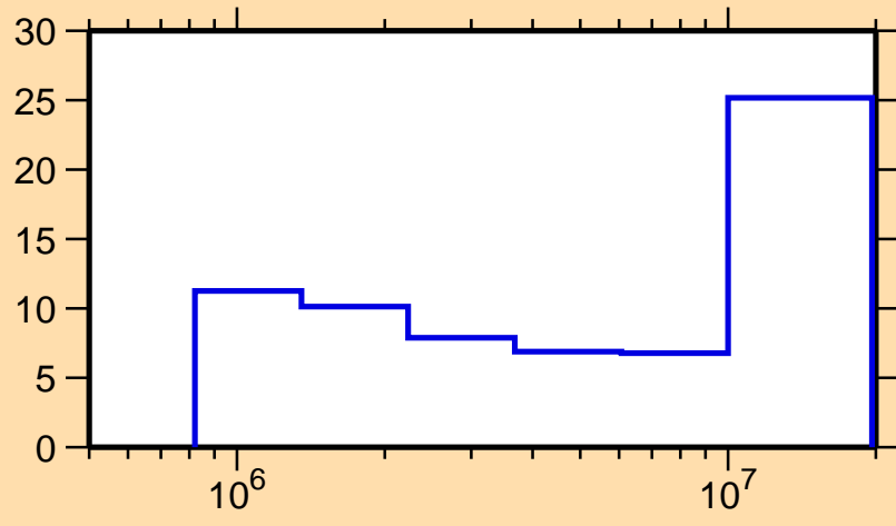
\Delta\sigma/\sigma vs. E for ^{114}\text{Sn}(n,\text{inel.})
