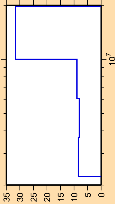
\Delta\sigma/\sigma vs. E for ^{114}\text{Sn}(n,n\text{cont.})
