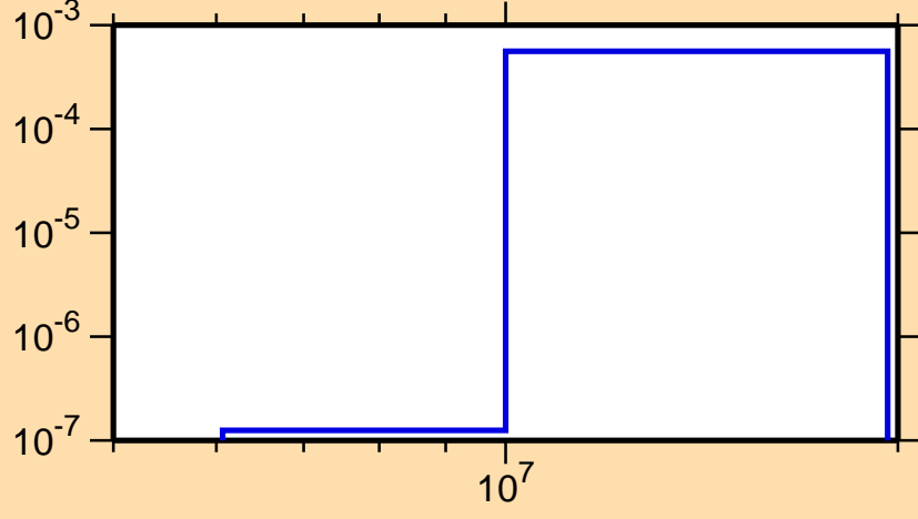
\sigma vs. E for ^{114}\text{Sn}(n,n\alpha)
