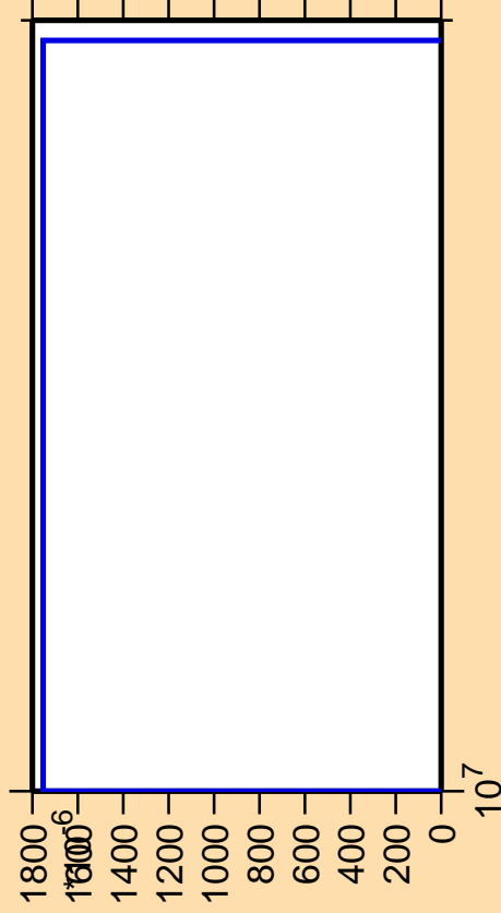
\Delta\sigma/\sigma vs. E for ^{114}\text{Sn}(\text{mt117})
