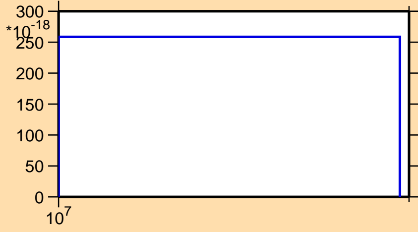
\sigma vs. E for ^{114}\text{Sn}(\text{mt117})
