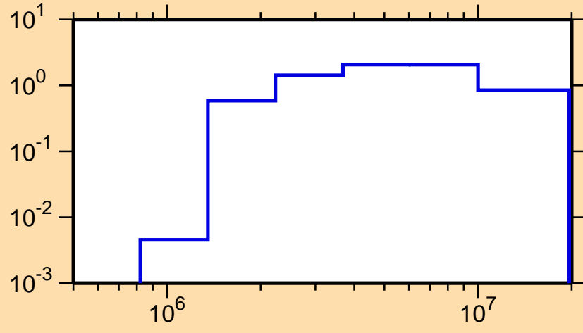
\sigma vs. E for ^{114}\text{Sn}(n,\text{inel.})
