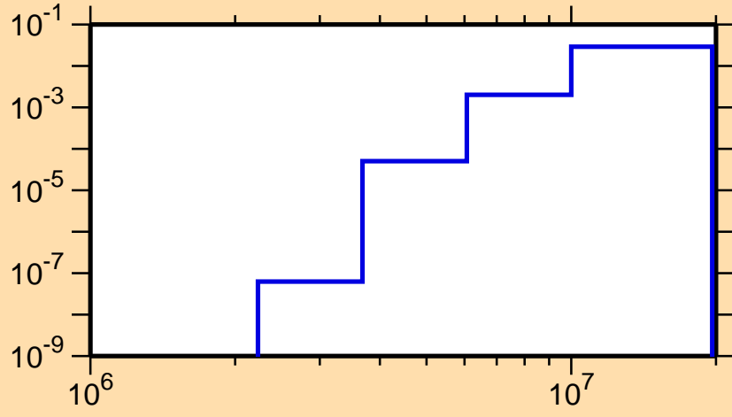
\sigma vs. E for ^{114}\text{Sn}(n,p)
