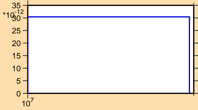
\sigma vs. E for ^{114}\text{Sn}(n,\text{nd})
