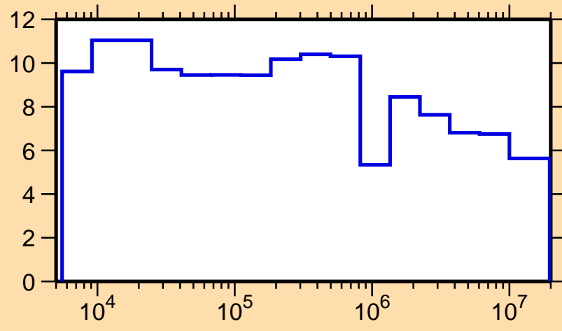
\Delta\sigma/\sigma vs. E for ^{114}\text{Sn}(n,\text{nonel.})
