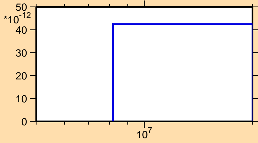
\sigma vs. E for ^{114}\text{Sn}(n,nd)
