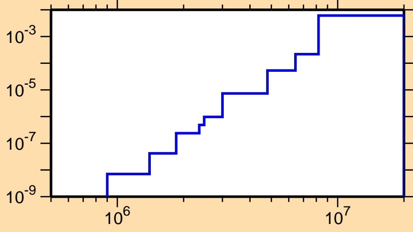
\sigma vs. E for ^{114}\text{Sn}(n,\alpha)
