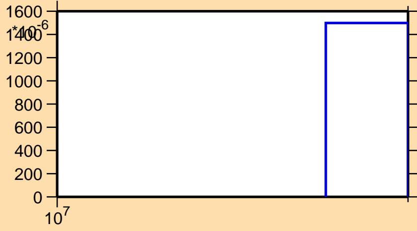
\sigma vs. E for ^{115}\text{Sn}(n,3n)
