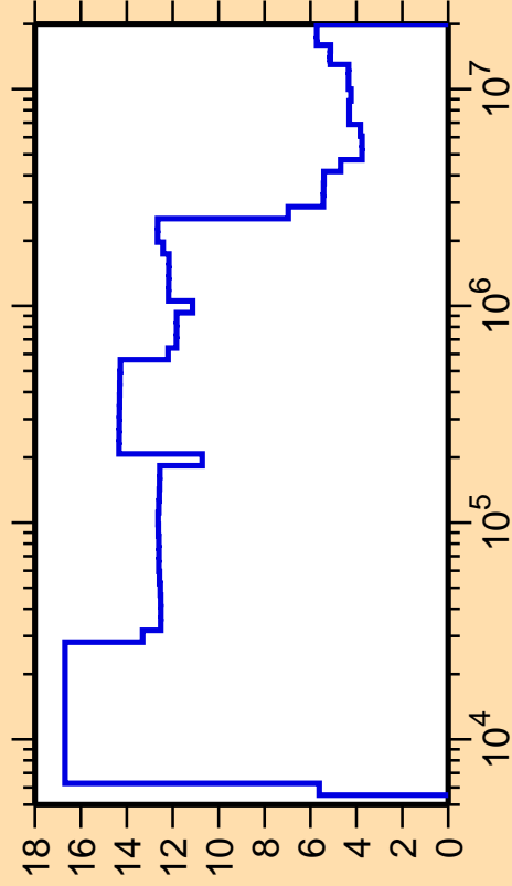
\Delta\sigma/\sigma vs. E for ^{115}\text{Sn}(n,\text{nonel.})
