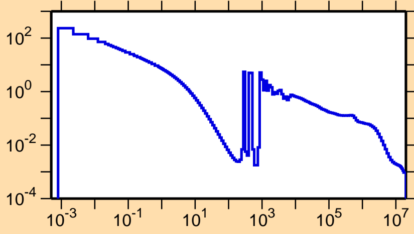
\sigma vs. E for ^{115}\text{Sn}(n,\gamma)
