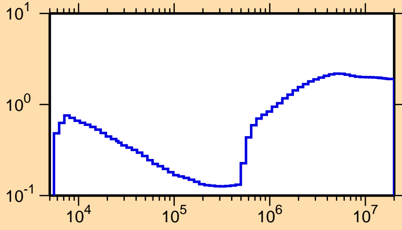
\sigma vs. E for ^{115}\text{Sn}(n,\text{nonel.})
