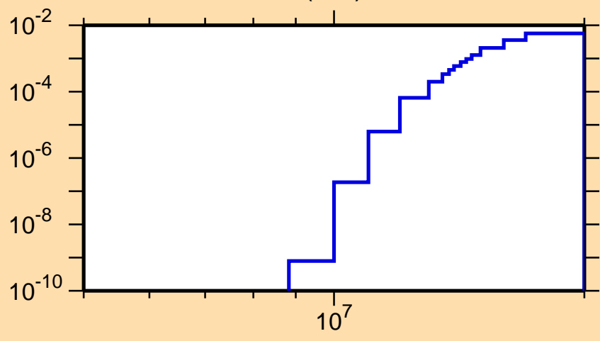
\sigma vs. E for ^{115}\text{Sn}(n,d)
