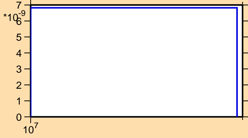
\sigma vs. E for ^{115}\text{Sn}(n,\text{nd})
