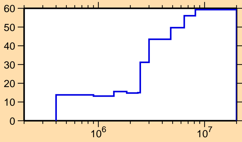
\Delta\sigma/\sigma vs. E for ^{115}\text{Sn}(n,n_1)
