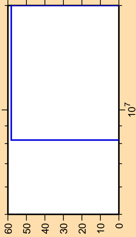
\Delta\sigma/\sigma vs. E for ^{115}\text{Sn}(n,np)
