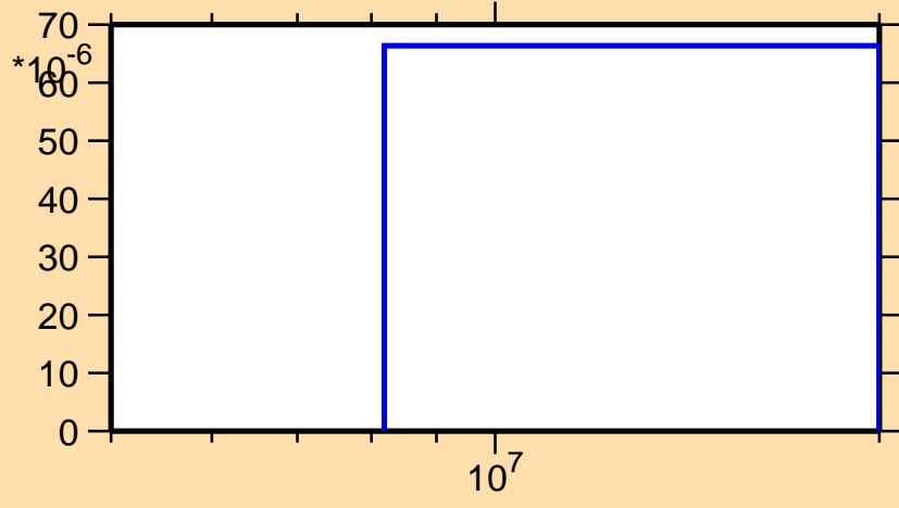
\sigma vs. E for ^{115}\text{Sn}(n,t)
