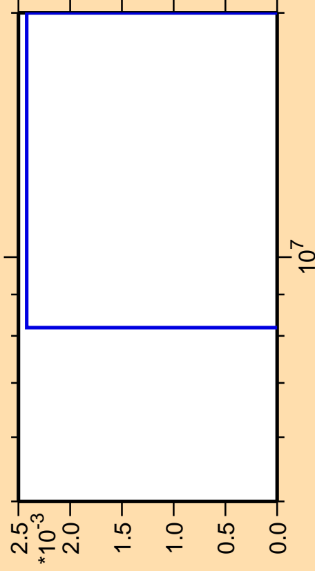
\Delta\sigma/\sigma vs. E for ^{115}\text{Sn}(n,\text{pt})
