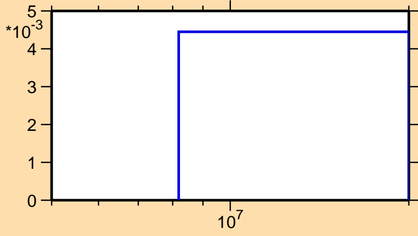
\sigma vs. E for ^{115}\text{Sn}(n,np)
