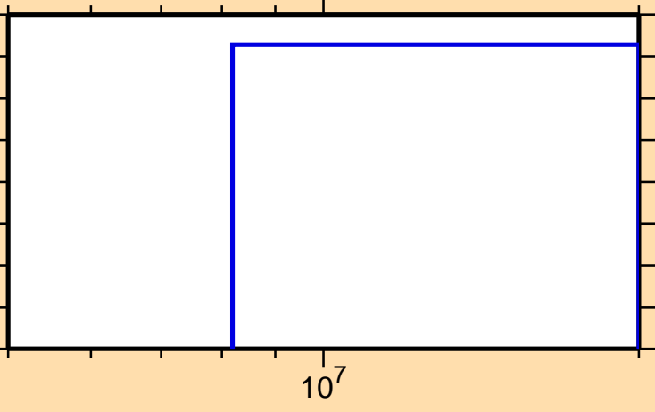
\sigma vs. E for ^{115}\text{Sn}(n,d)
