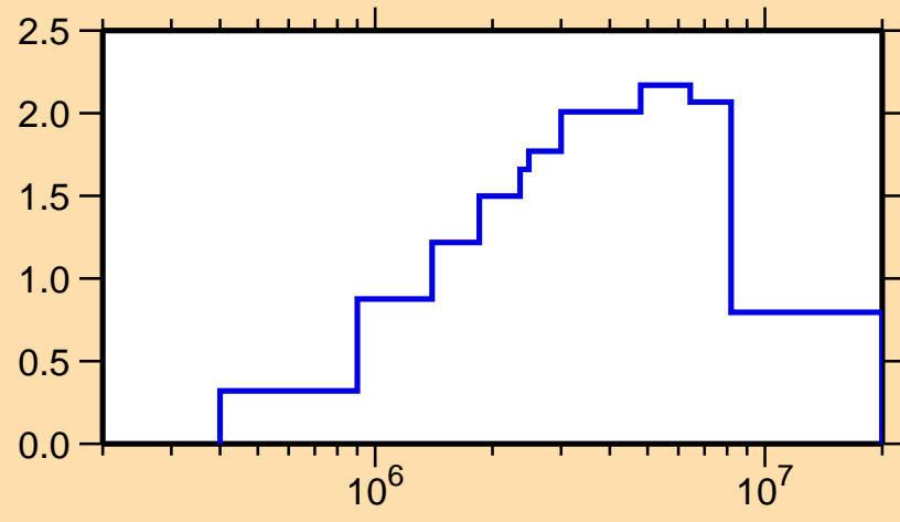
\sigma vs. E for ^{115}\text{Sn}(n,\text{inel.})
