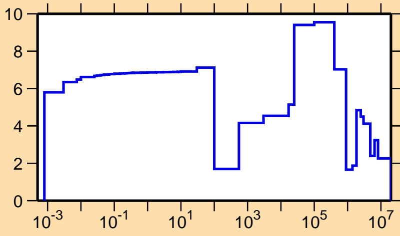
\Delta\sigma/\sigma vs. E for ^{116}\text{Sn}(n,\text{tot.})
