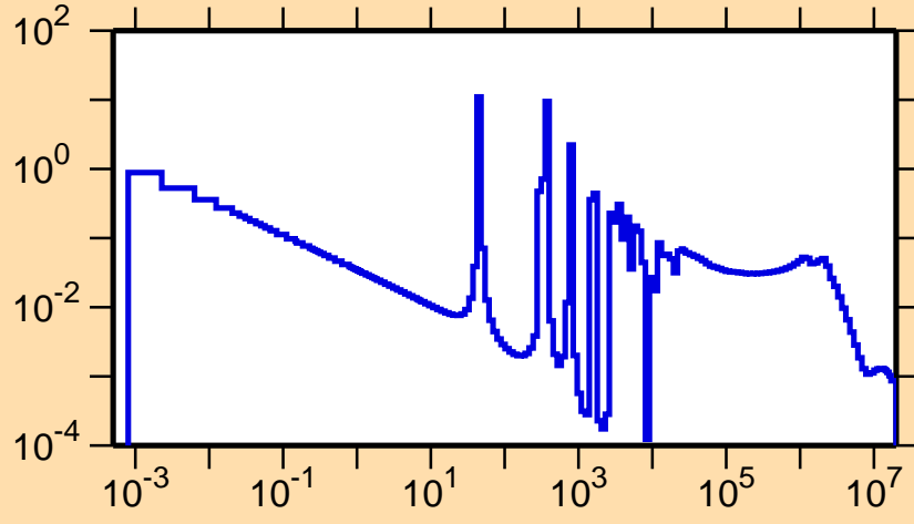
\sigma vs. E for ^{118}\text{Sn}(n,\gamma)
