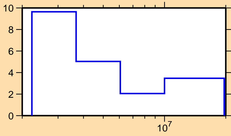
\Delta\sigma/\sigma vs. E for ^{118}\text{Sn}(n,\text{tot.})
