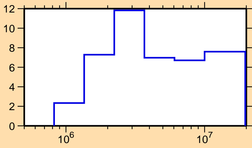
\Delta\sigma/\sigma vs. E for ^{118}\text{Sn}(n,\text{el.})
