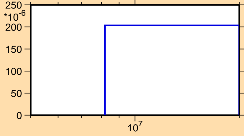
\sigma vs. E for ^{118}\text{Sn}(n,d)
