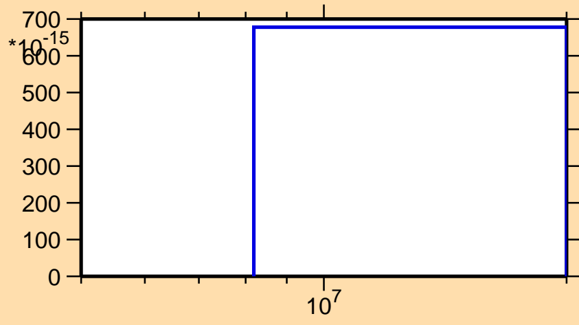
\sigma vs. E for ^{118}\text{Sn}(n,nd)
