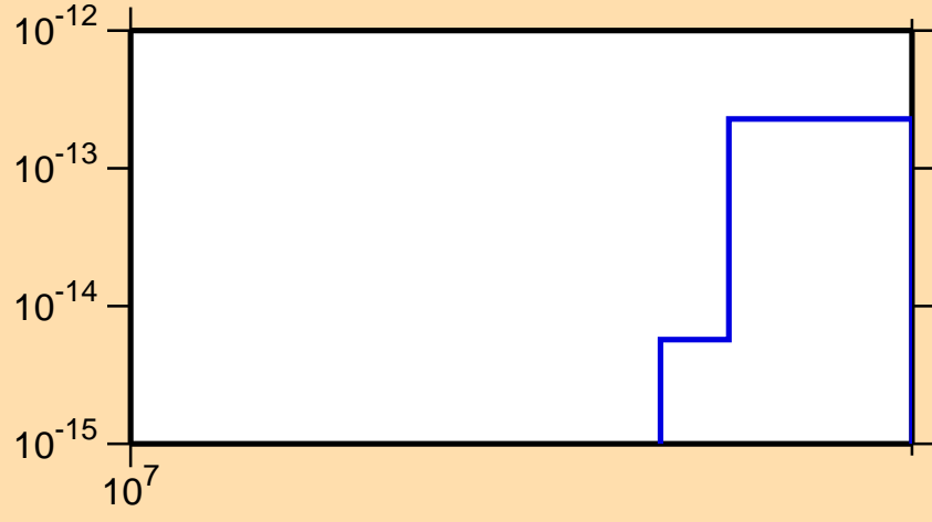
\sigma vs. E for ^{119}\text{Sn}(n,p\alpha)
