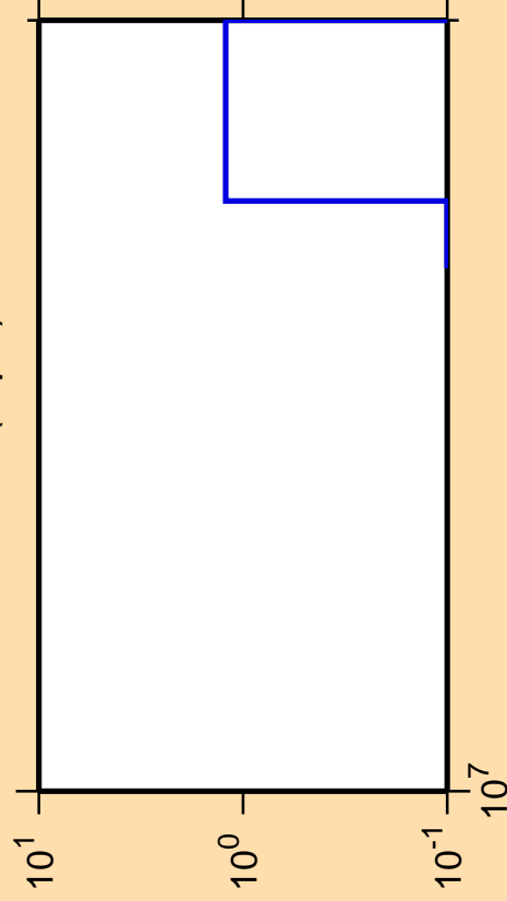
\Delta\sigma/\sigma vs. E for ^{119}\text{Sn}(n,p\alpha)
