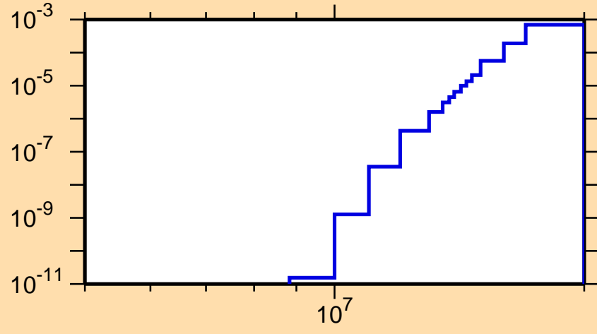
\sigma vs. E for ^{119}\text{Sn}(n,n\alpha)
