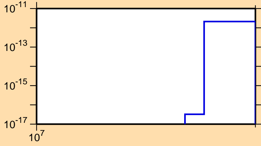
\sigma vs. E for ^{119}\text{Sn}(n,nt)
