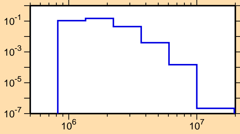
\sigma vs. E for ^{119}\text{Sn}(n,n_4)
