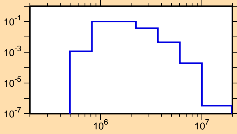
\sigma vs. E for ^{119}\text{Sn}(n,n_3)
