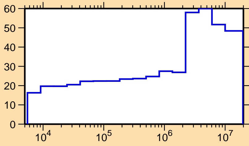
\Delta\sigma/\sigma vs. E for ^{119}\text{Sn}(n,\gamma)
