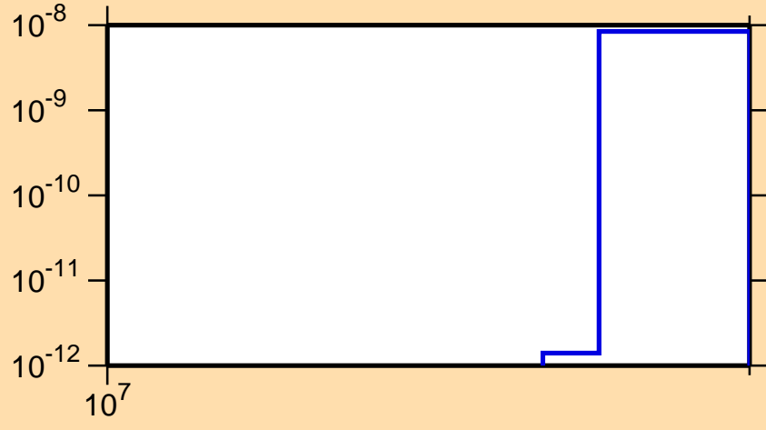
\sigma vs. E for ^{119}\text{Sn}(n,2np)
