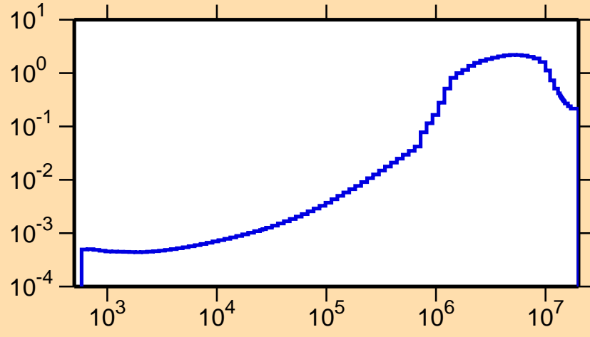
\sigma vs. E for ^{119}\text{Sn}(n,\text{inel.})
