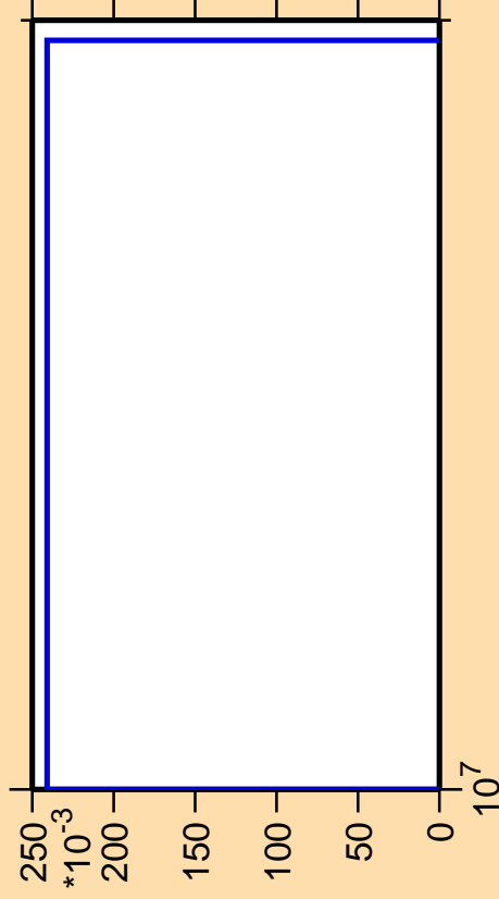
\Delta\sigma/\sigma vs. E for ^{119}\text{Sn}(n,\text{He}3)
