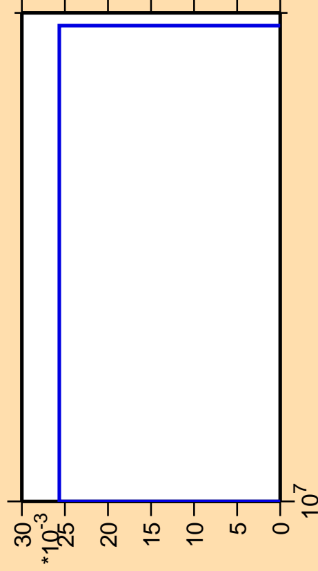
\Delta\sigma/\sigma vs. E for ^{119}\text{Sn}(n,p\alpha)
