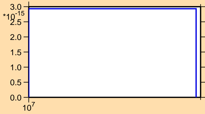
\sigma vs. E for ^{119}\text{Sn}(n,p\alpha)
