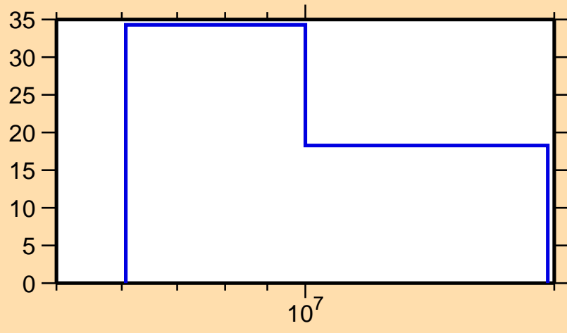
\Delta\sigma/\sigma vs. E for ^{119}\text{Sn}(n,2n)
