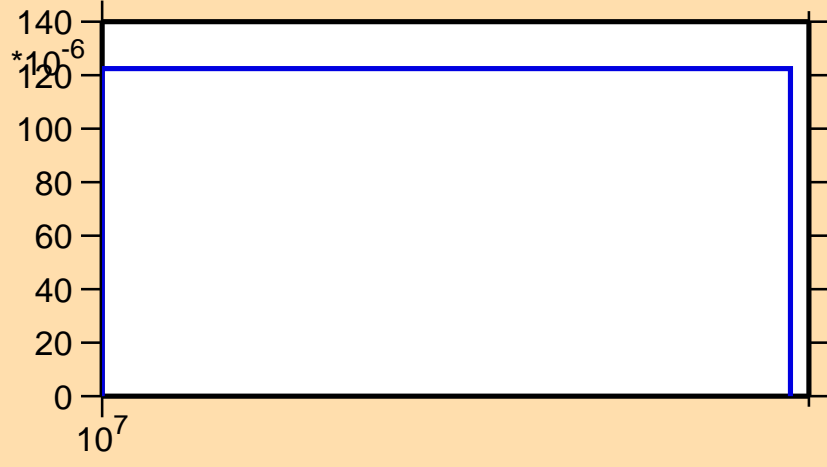
\sigma vs. E for ^{119}\text{Sn}(n,np)
