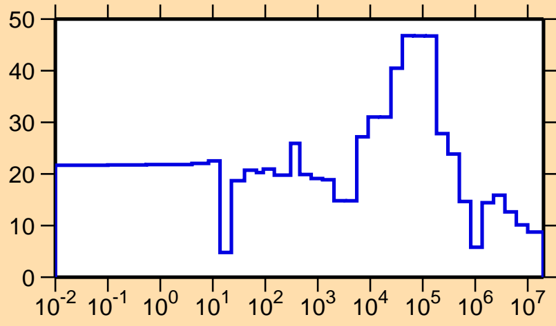
\Delta\sigma/\sigma vs. E for ^{119}\text{Sn}(n,\text{el.})
