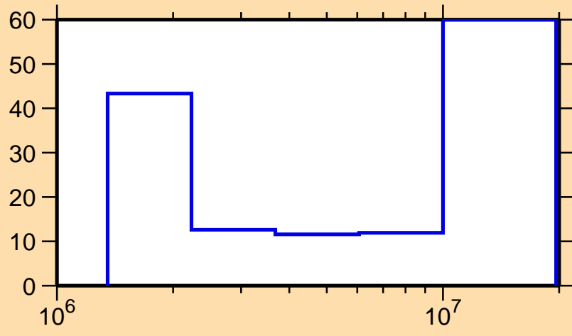
\Delta\sigma/\sigma vs. E for ^{119}\text{Sn}(n,n\text{cont.})
