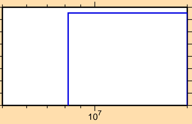
\sigma vs. E for ^{119}\text{Sn}(n,nt)
