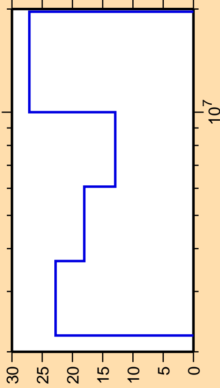
\Delta\sigma/\sigma vs. E for ^{120}\text{Sn}(n,n_{\text{cont}})
