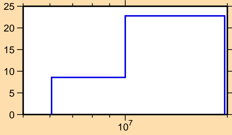
\Delta\sigma/\sigma vs. E for ^{120}\text{Sn}(n,\text{inel.})
