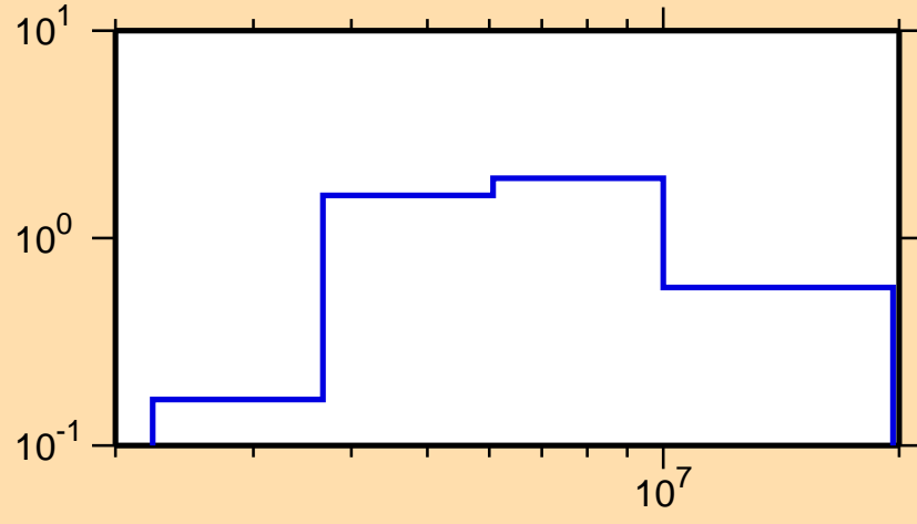
\sigma vs. E for ^{120}\text{Sn}(n,n\text{cont.})
