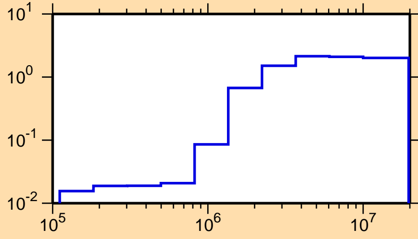
\sigma vs. E for ^{120}\text{Sn}(n,\text{nonel.})
