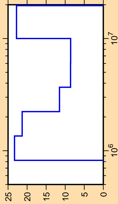
\Delta\sigma/\sigma vs. E for ^{120}\text{Sn}(n,\text{inel.})
