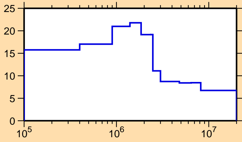
\Delta\sigma/\sigma vs. E for ^{120}\text{Sn}(n,\text{nonel.})
