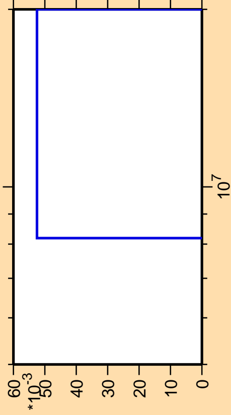
\Delta\sigma/\sigma vs. E for ^{120}\text{Sn}(n,2n\alpha)
