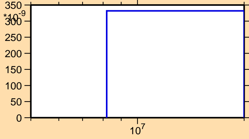
\sigma vs. E for ^{120}\text{Sn}(n,t)
