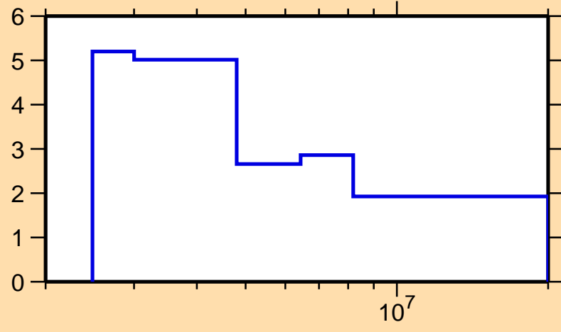
\Delta\sigma/\sigma vs. E for ^{120}\text{Sn}(n,\text{tot.})
