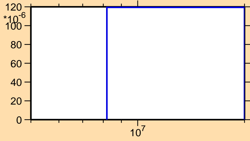
\sigma vs. E for ^{120}\text{Sn}(n,d)
