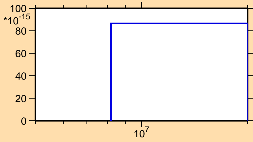
\sigma vs. E for ^{120}\text{Sn}(n,nd)
