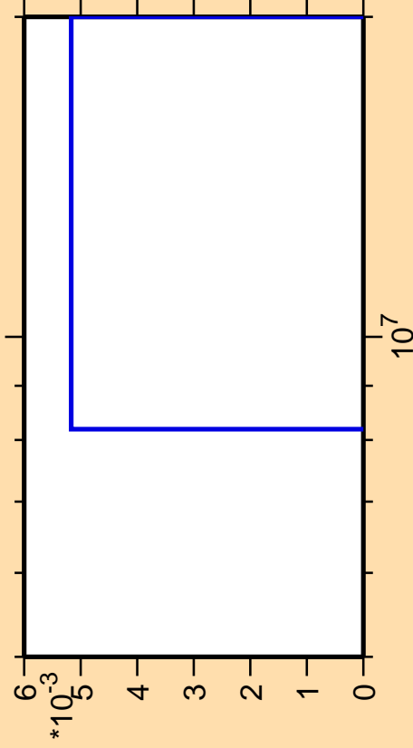
\Delta\sigma/\sigma vs. E for ^{120}\text{Sn}(n,nt)
