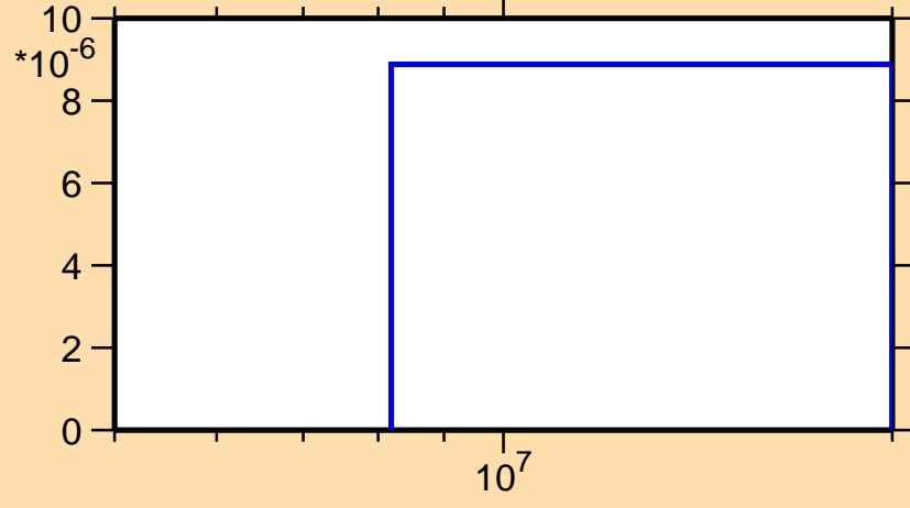
\sigma vs. E for ^{120}\text{Sn}(n,n\alpha)
