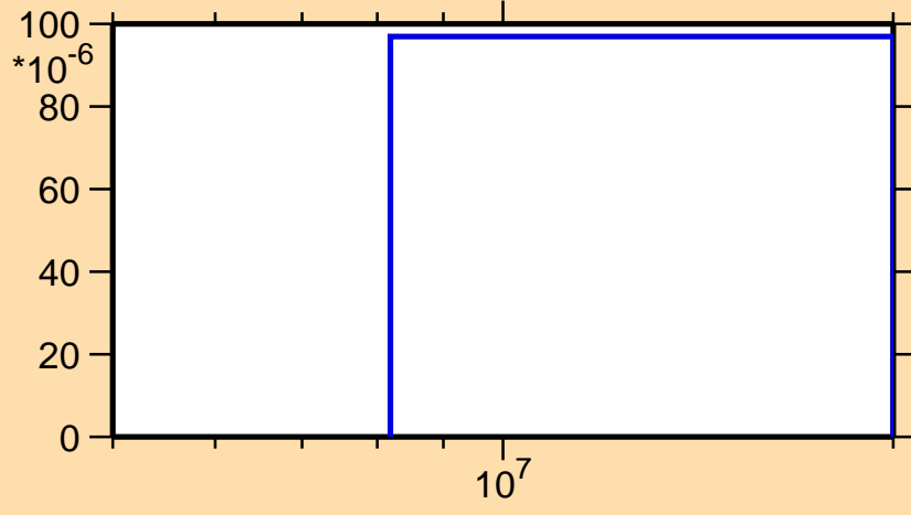
\sigma vs. E for ^{120}\text{Sn}(n,np)
