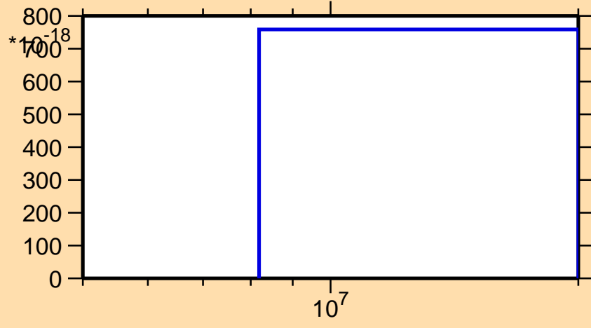
\sigma vs. E for ^{120}\text{Sn}(n,nt)
