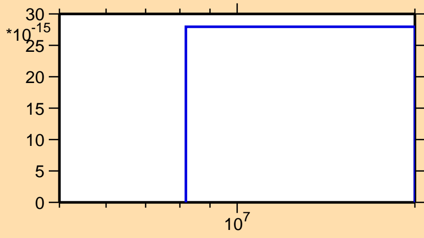
\sigma vs. E for ^{120}\text{Sn}(n,2n\alpha)
