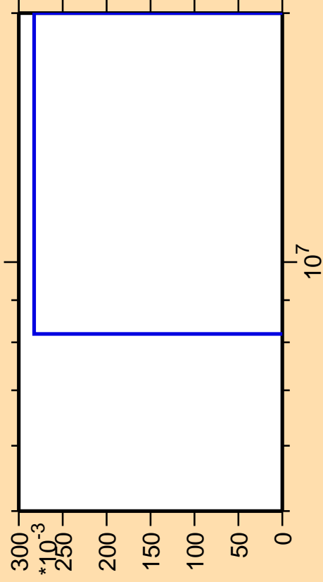
\Delta\sigma/\sigma vs. E for ^{120}\text{Sn}(n,nd)
