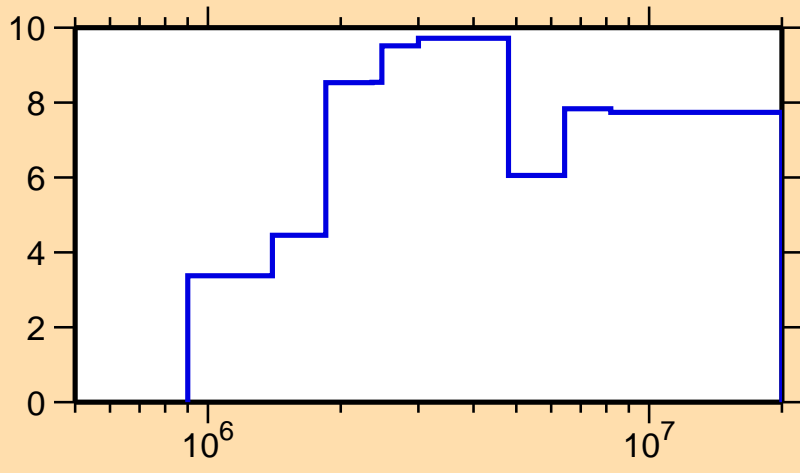
\Delta\sigma/\sigma vs. E for ^{120}\text{Sn}(n,\text{el.})
