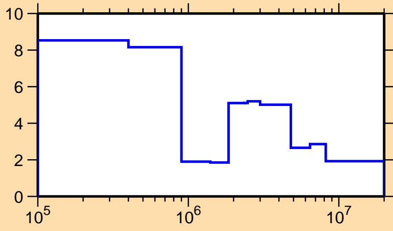
\Delta\sigma/\sigma vs. E for ^{120}\text{Sn}(n,\text{tot.})
