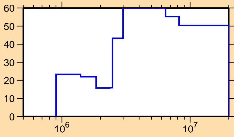
\Delta\sigma/\sigma vs. E for ^{120}\text{Sn}(n,n_1)
