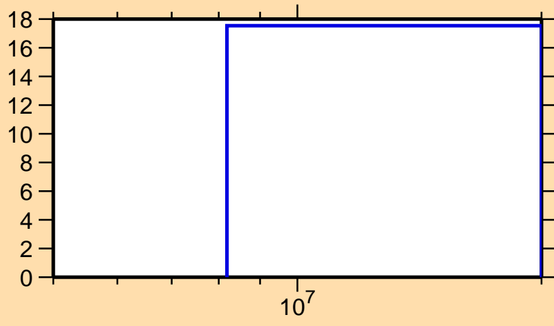
\Delta\sigma/\sigma vs. E for ^{120}\text{Sn}(n,\text{inel.})
