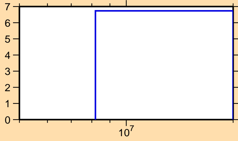
\Delta\sigma/\sigma vs. E for ^{120}\text{Sn}(n,\text{nonel.})
