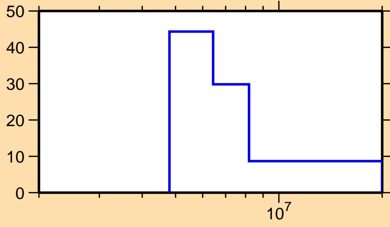
\Delta\sigma/\sigma vs. E for ^{121}\text{Sn}(n,2n)
