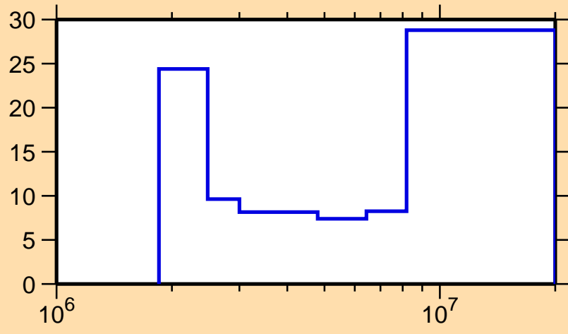
\Delta\sigma/\sigma vs. E for ^{121}\text{Sn}(n,n\text{cont.})
