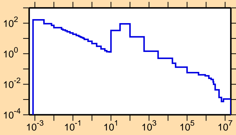
\sigma vs. E for ^{121}\text{Sn}(n,\gamma)
