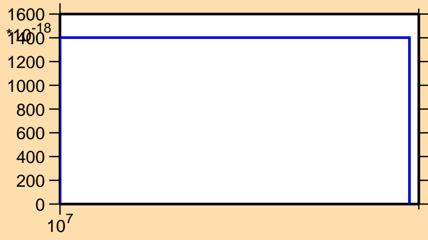
\sigma vs. E for ^{122}\text{Sn}(n,nd)
