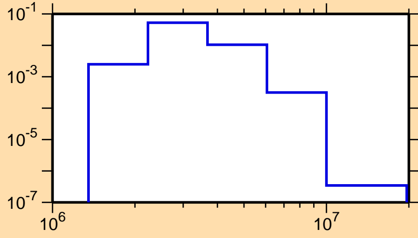
\sigma vs. E for ^{122}\text{Sn}(n,n_2)
