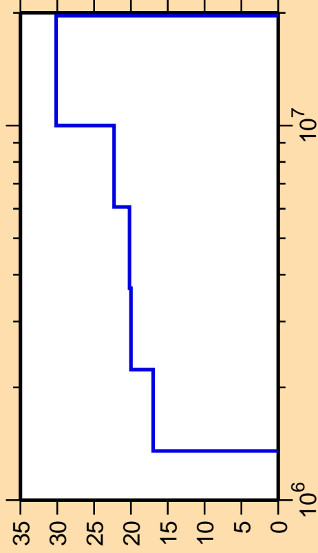
\Delta\sigma/\sigma vs. E for ^{122}\text{Sn}(n,n_4)
