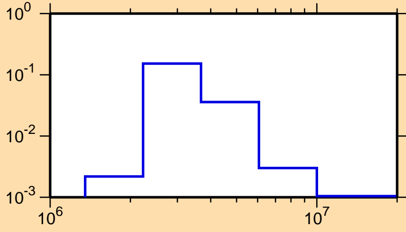
\sigma vs. E for ^{122}\text{Sn}(n,n_4)
