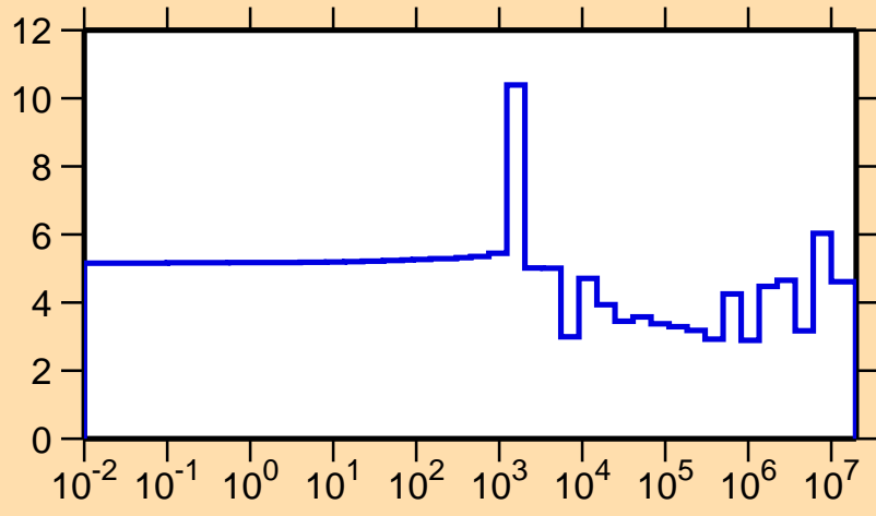
\Delta\sigma/\sigma vs. E for ^{122}\text{Sn}(n,\text{el.})
