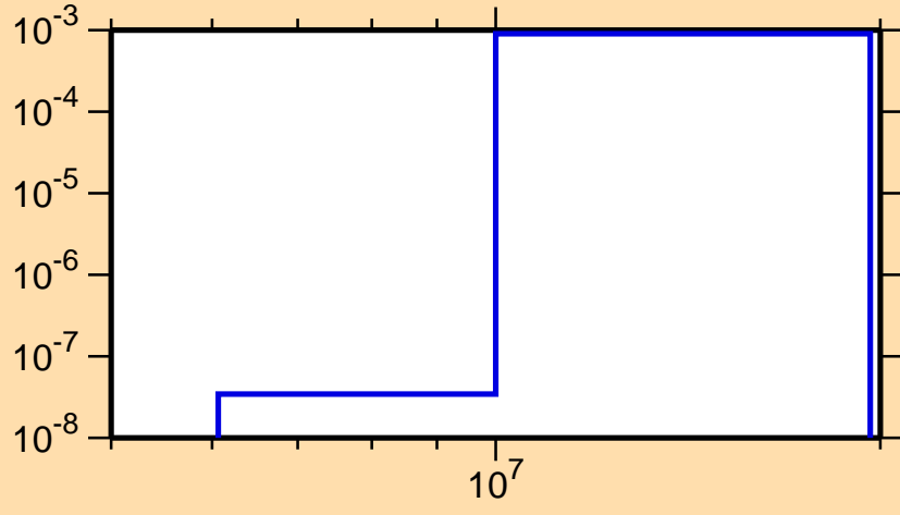
\sigma vs. E for ^{122}\text{Sn}(n,p)
