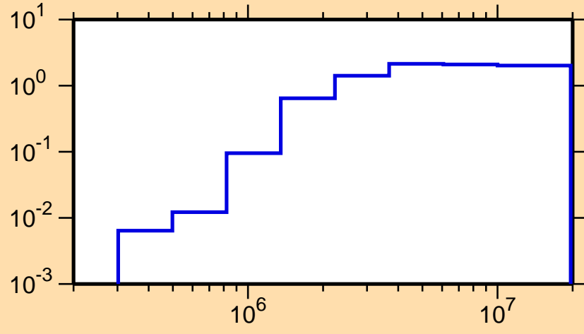
\sigma vs. E for ^{122}\text{Sn}(n,\text{nonel.})
