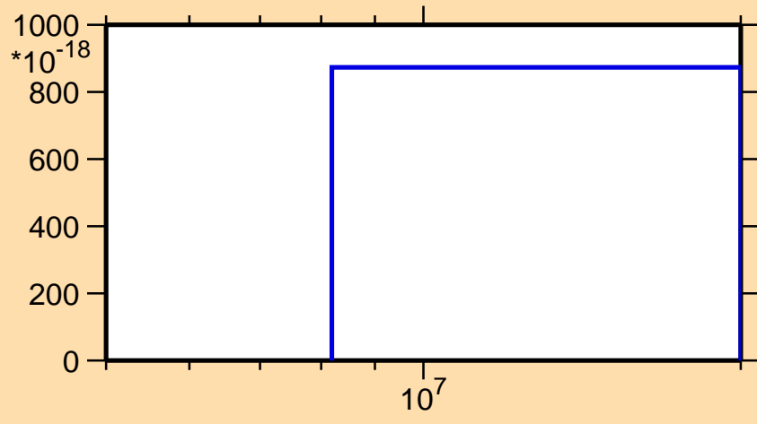
\sigma vs. E for ^{122}\text{Sn}(n,2n\alpha)
