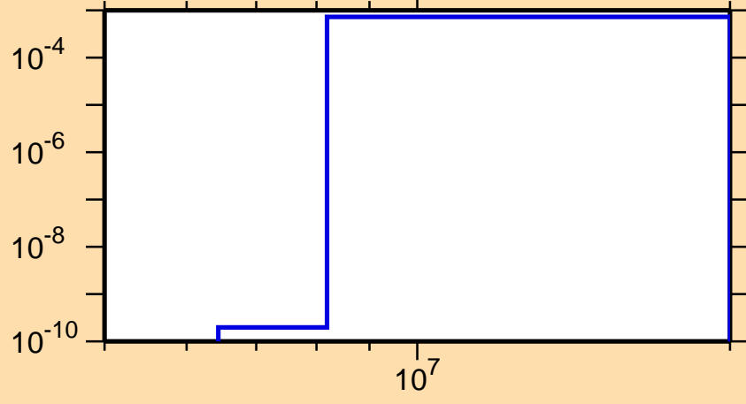
\sigma vs. E for ^{122}\text{Sn}(n,p)
