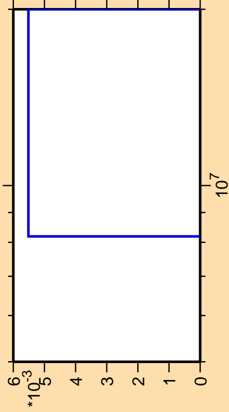
\Delta\sigma/\sigma vs. E for ^{122}\text{Sn}(n,2n\alpha)
