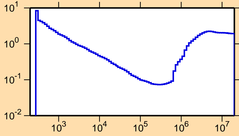
\sigma vs. E for ^{123}\text{Sn}(n,\text{nonel.})
