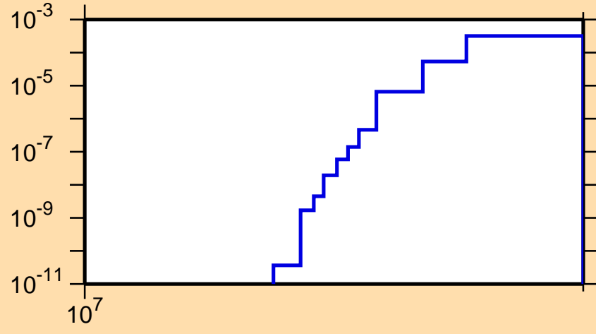
\sigma vs. E for ^{123}\text{Sn}(n,np)
