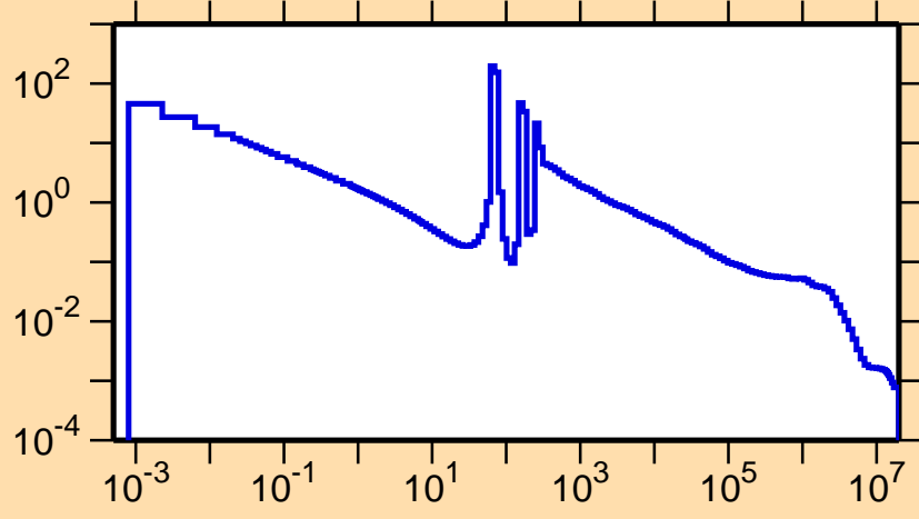
\sigma vs. E for ^{123}\text{Sn}(n,\gamma)
