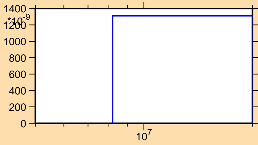
\sigma vs. E for ^{123}\text{Sn}(n,t)
