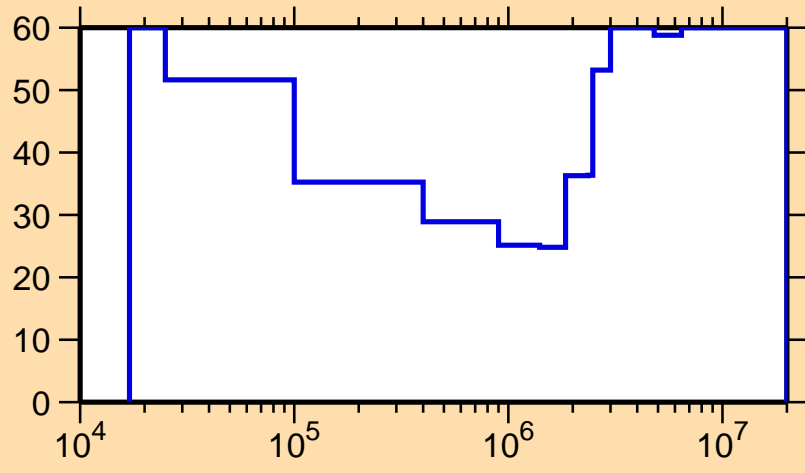
\Delta\sigma/\sigma vs. E for ^{123}\text{Sn}(n,n_1)
