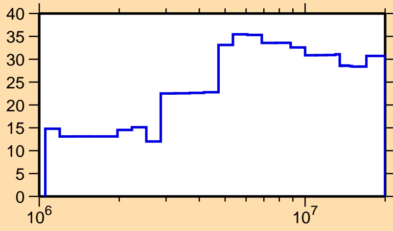
\Delta\sigma/\sigma vs. E for ^{124}\text{Sn}(n,n_1)
