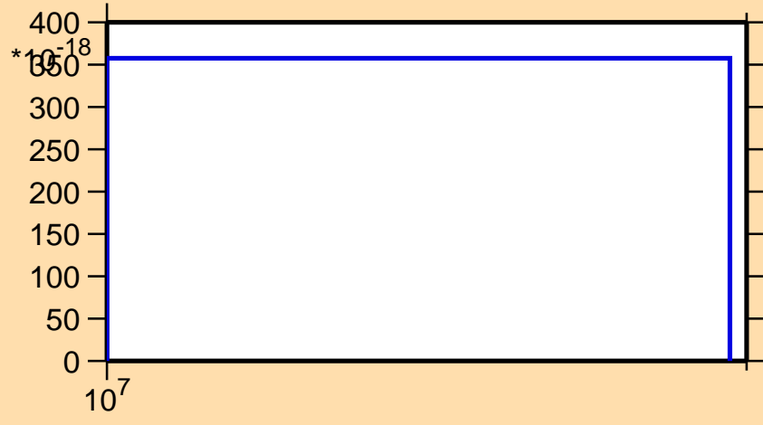
\sigma vs. E for ^{124}\text{Sn}(n,nd)
