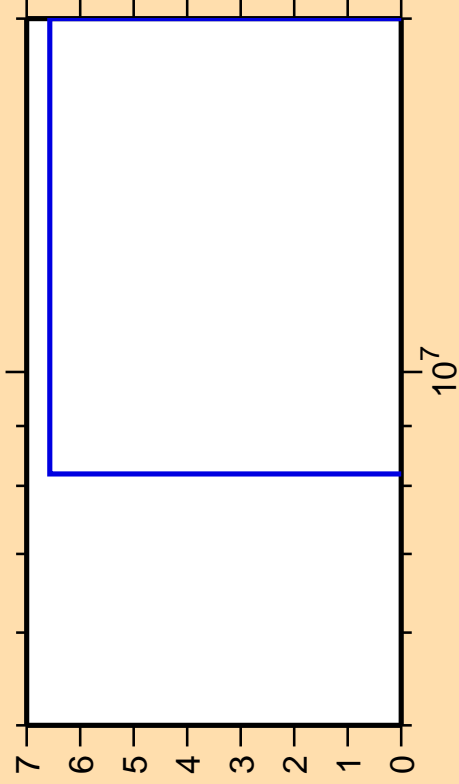
\Delta\sigma/\sigma vs. E for ^{124}\text{Sn}(n,2n)
