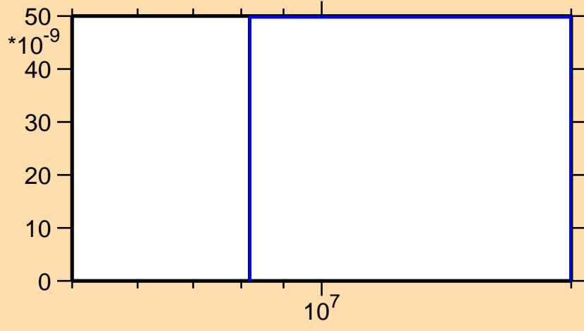
\sigma vs. E for ^{124}\text{Sn}(n,t)
