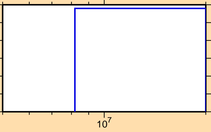
\sigma vs. E for ^{124}\text{Sn}(n,3n)
