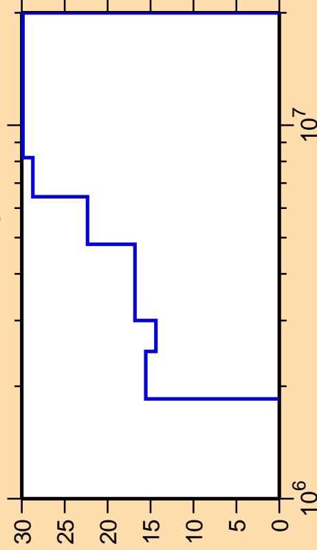
\Delta\sigma/\sigma vs. E for ^{124}\text{Sn}(n,n_3)
