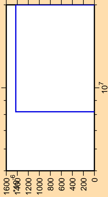
\Delta\sigma/\sigma vs. E for ^{124}\text{Sn}(n,nd)
