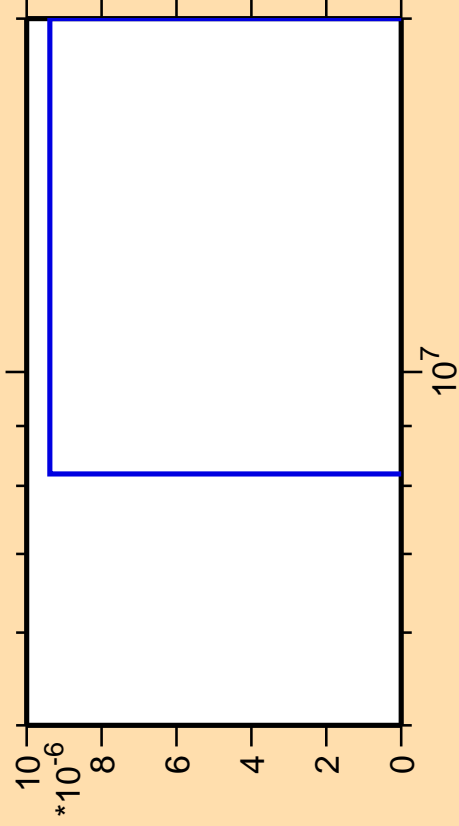
\Delta\sigma/\sigma vs. E for ^{124}\text{Sn}(n,2n\alpha)
