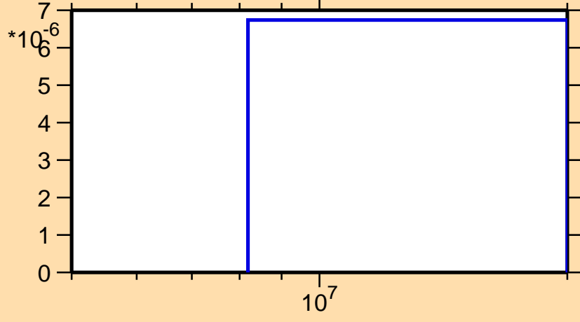
\sigma vs. E for ^{124}\text{Sn}(n,d)
