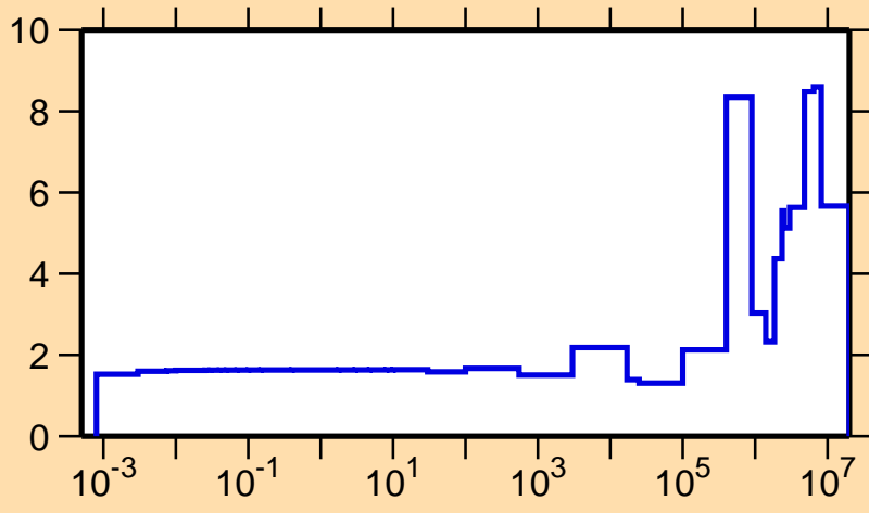
\Delta\sigma/\sigma vs. E for ^{124}\text{Sn}(n,\text{el.})
