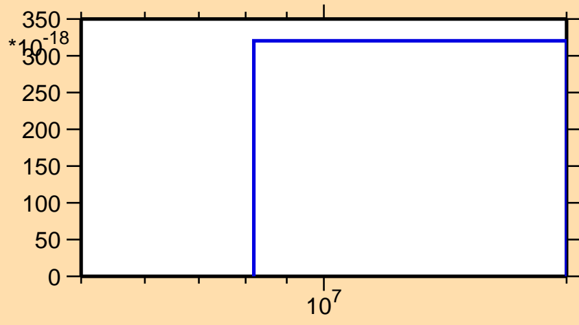
\sigma vs. E for ^{124}\text{Sn}(n,nd)
