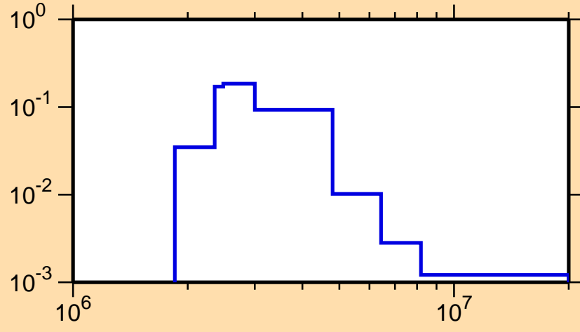
\sigma vs. E for ^{124}\text{Sn}(n,n_3)
