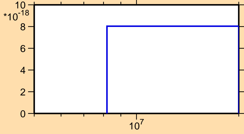
\sigma vs. E for ^{124}\text{Sn}(n,2n\alpha)
