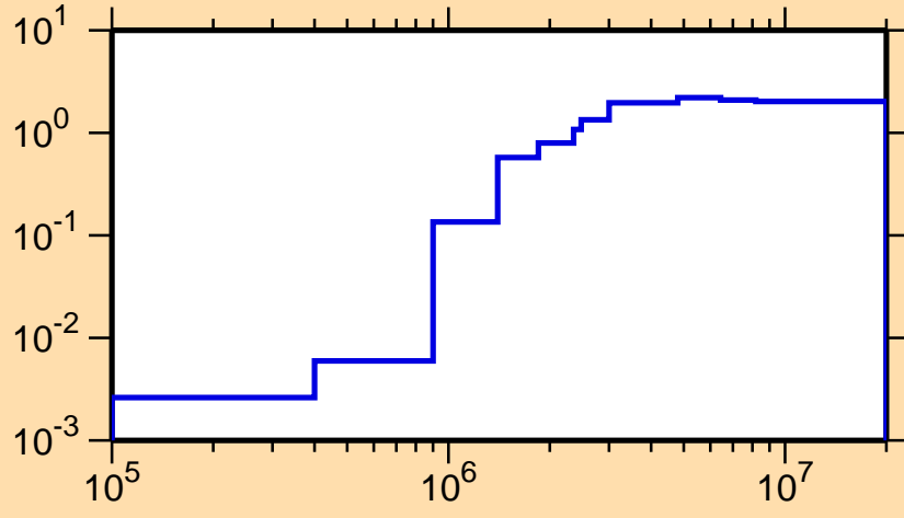
\sigma vs. E for ^{124}\text{Sn}(n,\text{nonel.})
