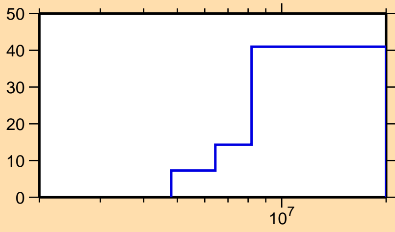
\Delta\sigma/\sigma vs. E for ^{125}\text{Sn}(n,n\text{cont.})
