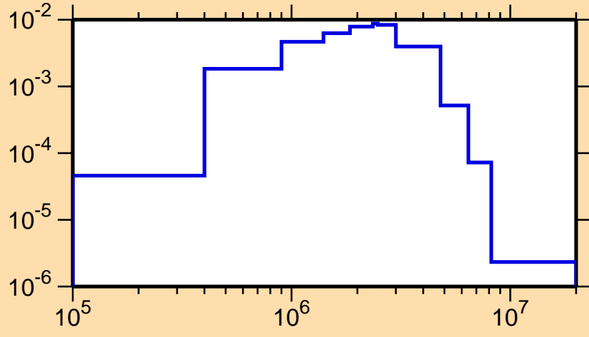
\sigma vs. E for ^{125}\text{Sn}(n,n_2)
