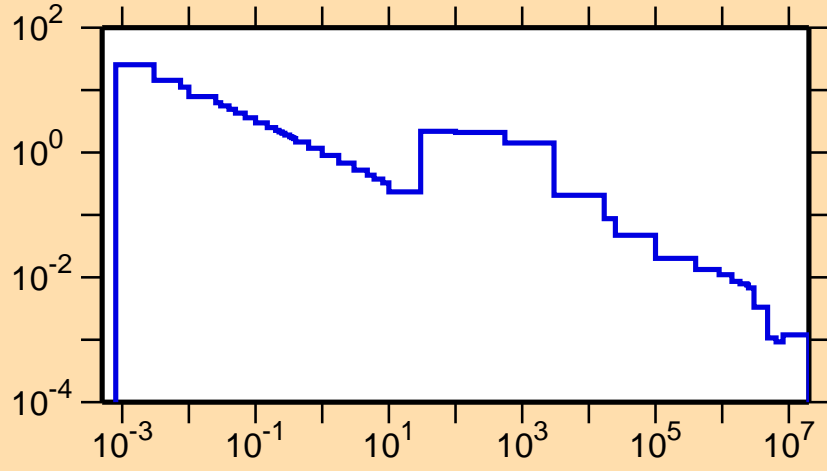
\sigma vs. E for ^{125}\text{Sn}(n,\gamma)
