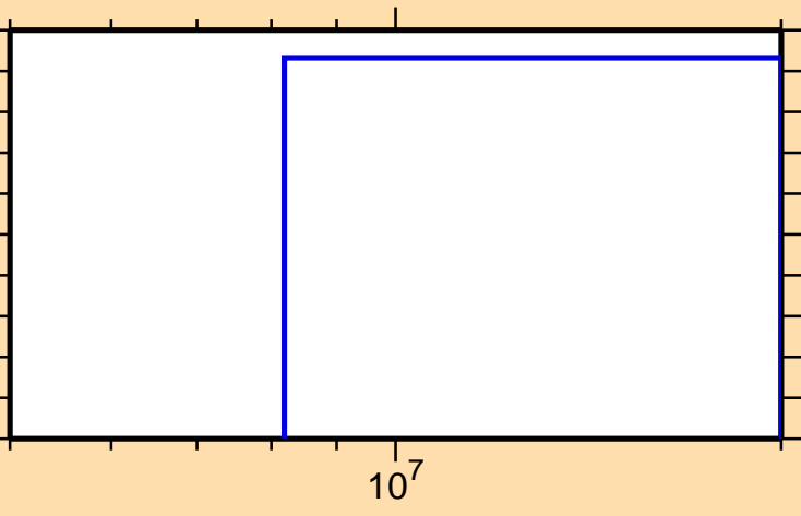
\sigma vs. E for ^{125}\text{Sn}(n,3n)
