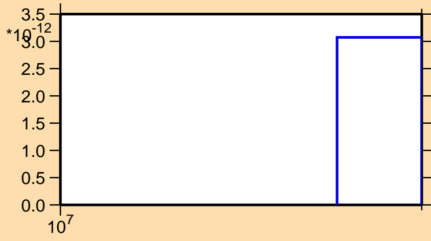
\sigma vs. E for ^{125}\text{Sn}(n,2np)
