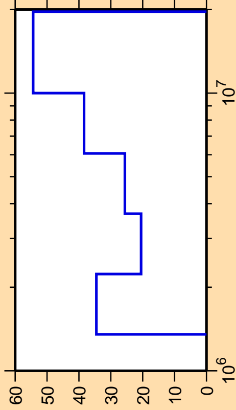
\Delta\sigma/\sigma vs. E for ^{126}\text{Sn}(n,n_4)
