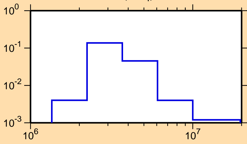
\sigma vs. E for ^{126}\text{Sn}(n,n_4)
