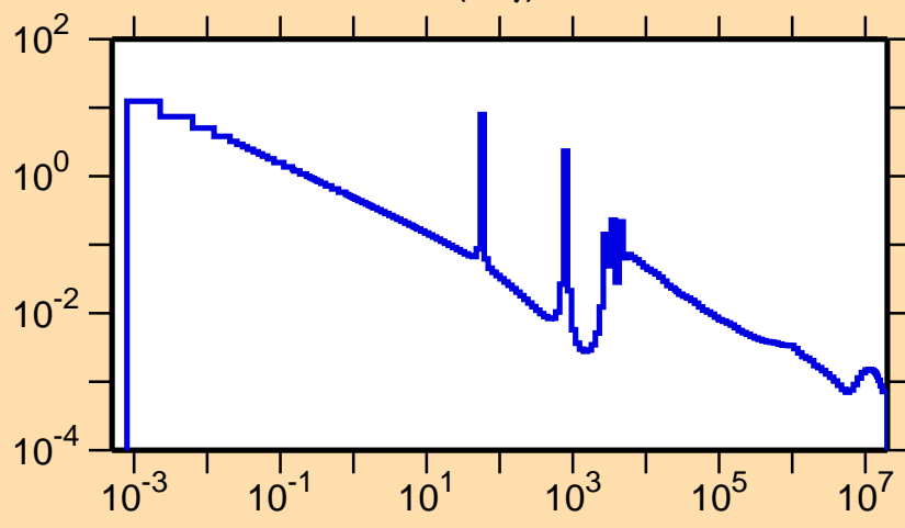
\sigma vs. E for ^{127}\text{Sn}(n,\gamma)
