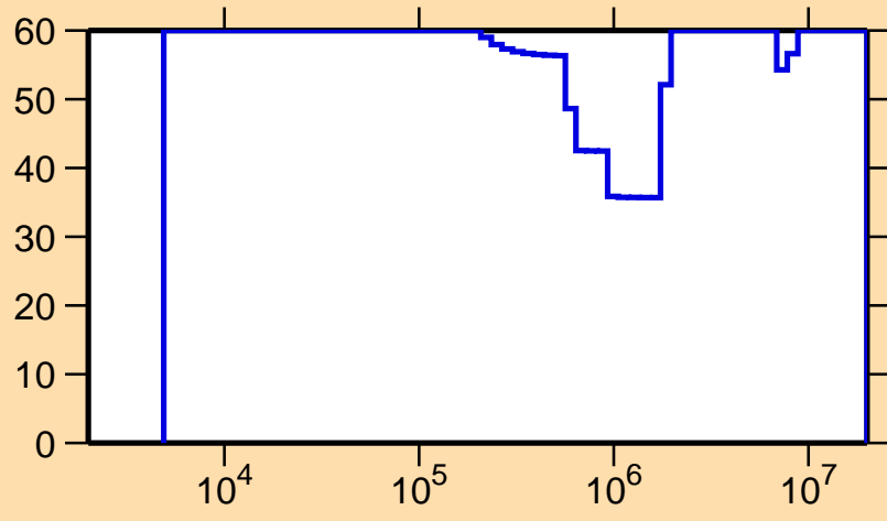
\Delta\sigma/\sigma vs. E for ^{127}\text{Sn}(n,n_1)
