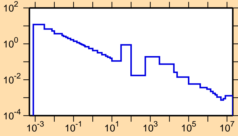
\sigma vs. E for ^{127}\text{Sn}(n,\gamma)
