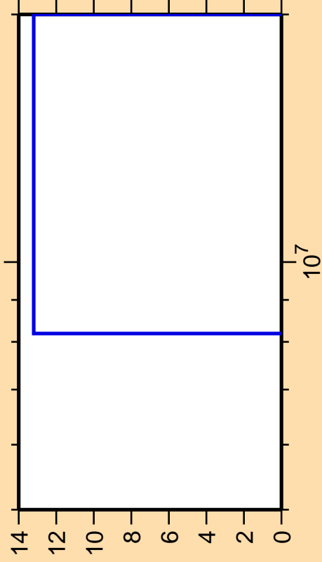
\Delta\sigma/\sigma vs. E for ^{127}\text{Sn}(n,nd)
