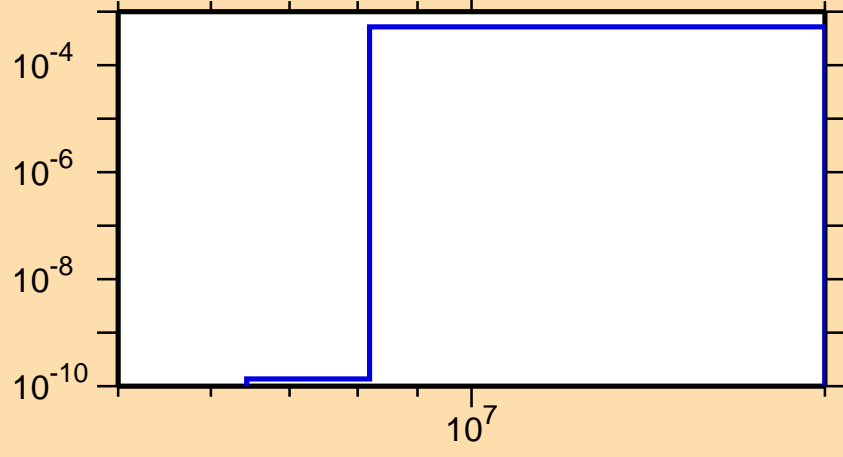
\sigma vs. E for ^{127}\text{Sn}(n,p)
