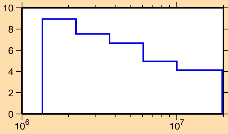
\Delta\sigma/\sigma vs. E for ^{127}\text{Sn}(n,\text{nonel.})
