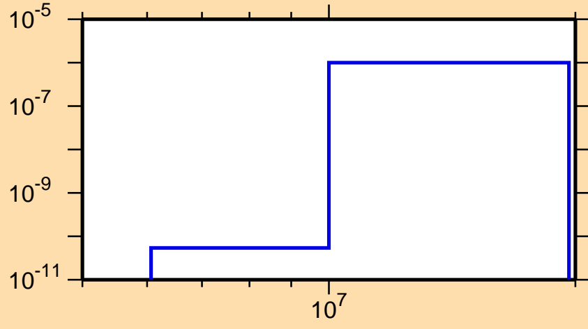
\sigma vs. E for ^{127}\text{Sn}(n,\alpha)
