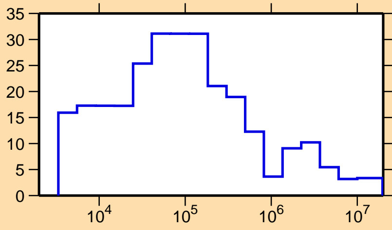
\Delta\sigma/\sigma vs. E for ^{127}\text{Sn}(n,\text{tot.})
