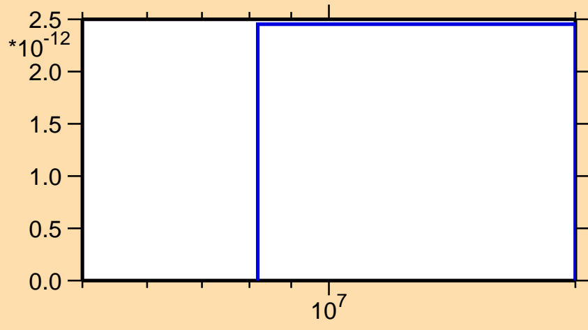
\sigma vs. E for ^{127}\text{Sn}(n,nd)
