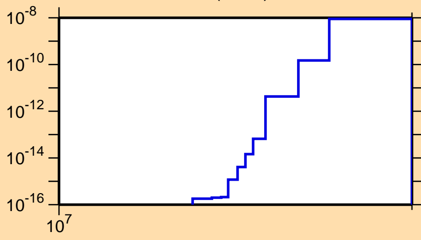
\sigma vs. E for ^{129}\text{Sn}(n,\alpha)
