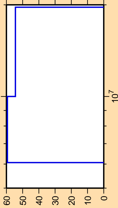
\Delta\sigma/\sigma vs. E for ^{129}\text{Sn}(n,p)
