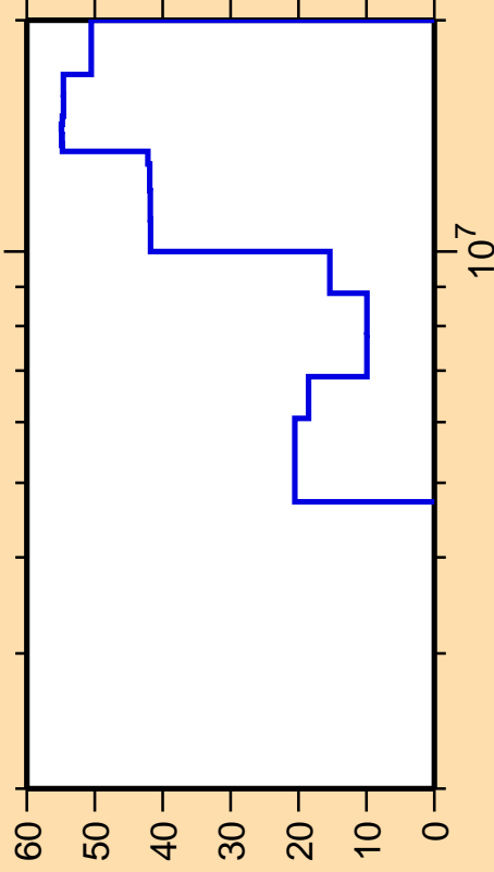
\Delta\sigma/\sigma vs. E for ^{130}\text{Sn}(n,n_{\text{cont}}) .
