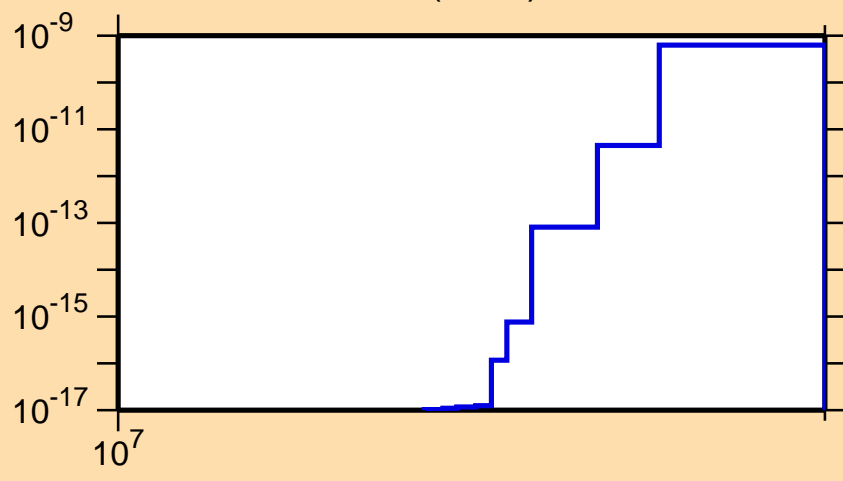
\sigma vs. E for ^{130}\text{Sn}(n,n\alpha)
