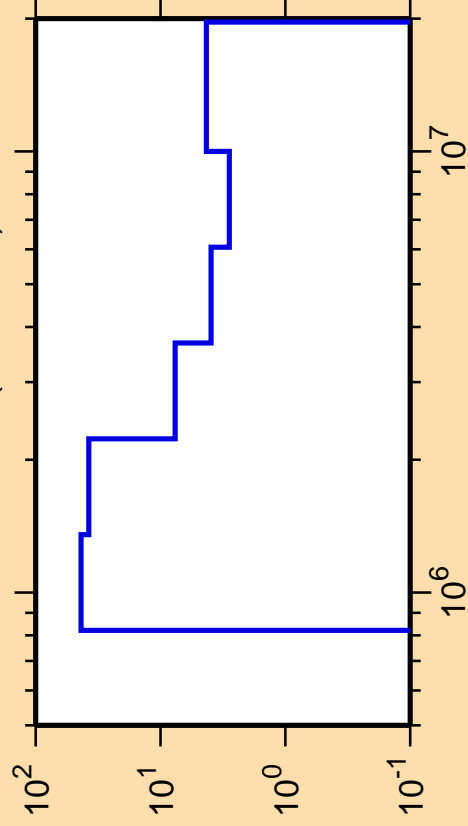
\Delta\sigma/\sigma vs. E for ^{130}\text{Sn}(n,\text{nonel.})
