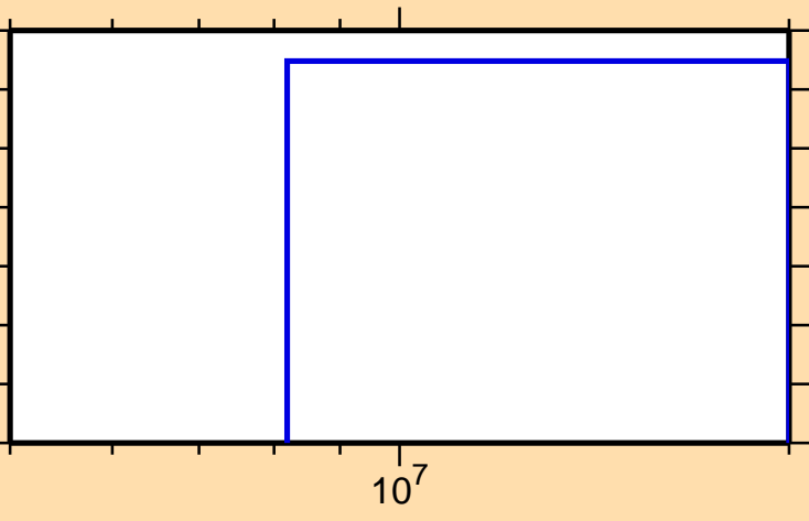
\sigma vs. E for ^{130}\text{Sn}(n,nd)
