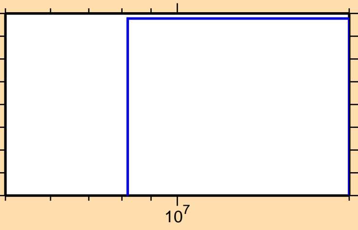
\sigma vs. E for ^{131}\text{Sn}(n,p)
