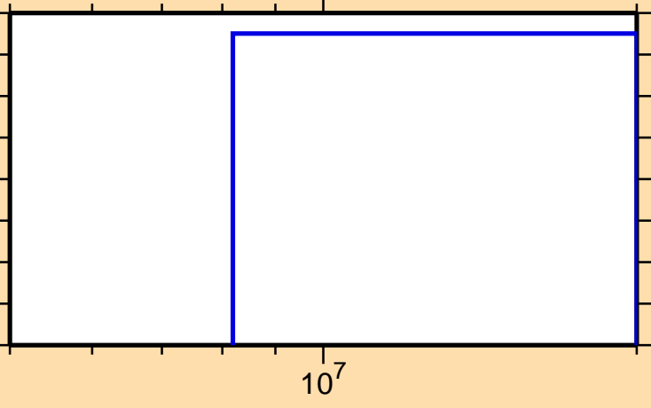
\sigma vs. E for ^{131}\text{Sn}(n,\alpha)
