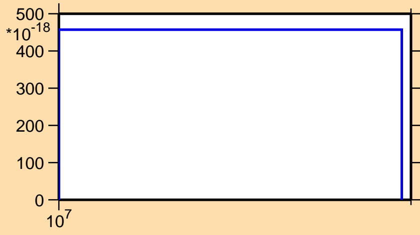
\sigma vs. E for ^{131}\text{Sn}(n,\text{nd})
