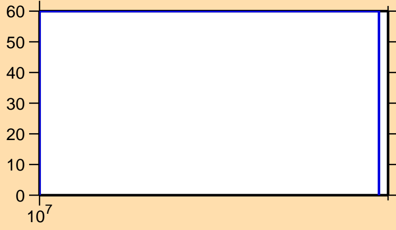
\Delta\sigma/\sigma vs. E for ^{132}\text{Sn}(n,p)
