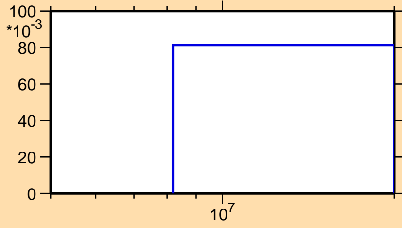
\sigma vs. E for ^{132}\text{Sn}(n,3n)
