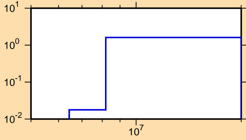
\sigma vs. E for ^{132}\text{Sn}(n,2n)
