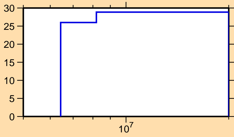
\Delta\sigma/\sigma vs. E for ^{132}\text{Sn}(n,\text{nonel.})
