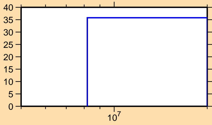
\Delta\sigma/\sigma vs. E for ^{132}\text{Sn}(n,\text{tot.})
