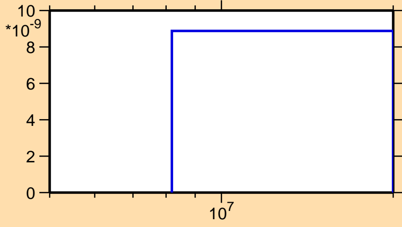
\sigma vs. E for ^{132}\text{Sn}(n,p)
