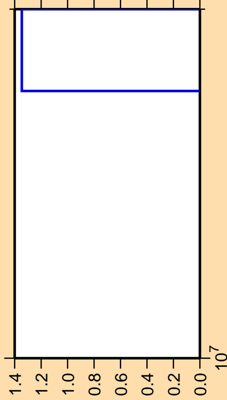
\Delta\sigma/\sigma vs. E for ^{133}\text{Sn}(n,\text{nd})
