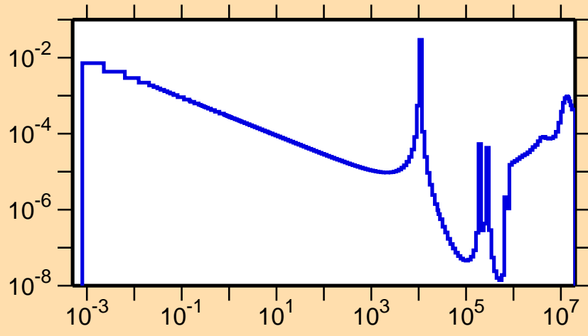
\sigma vs. E for ^{133}\text{Sn}(n,\gamma)
