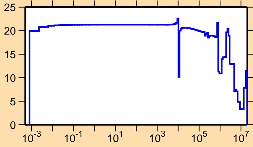
\Delta\sigma/\sigma vs. E for ^{133}\text{Sn}(n,\text{tot.})
