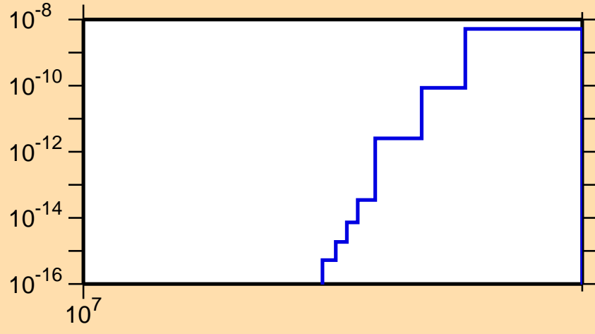
\sigma vs. E for ^{133}\text{Sn}(n,n\alpha)
