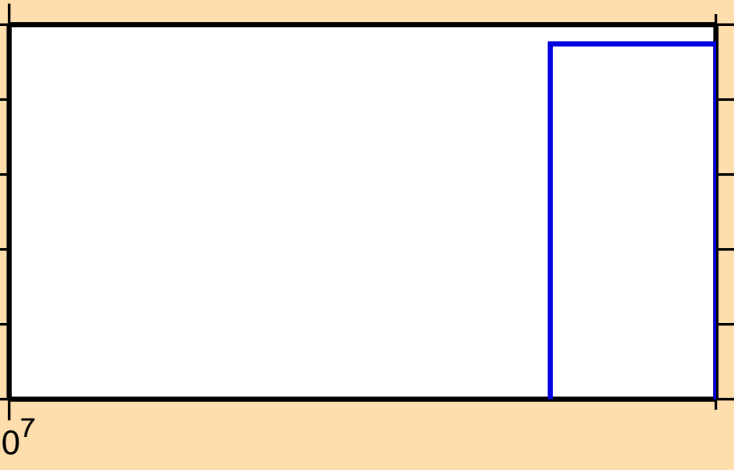
\sigma vs. E for ^{133}\text{Sn}(n,\text{nd})
