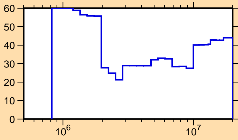
\Delta\sigma/\sigma vs. E for ^{133}\text{Sn}(n,\text{inel.})
