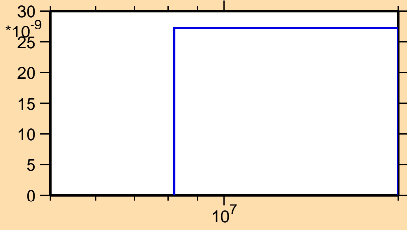
\sigma vs. E for ^{133}\text{Sn}(n,\alpha)
