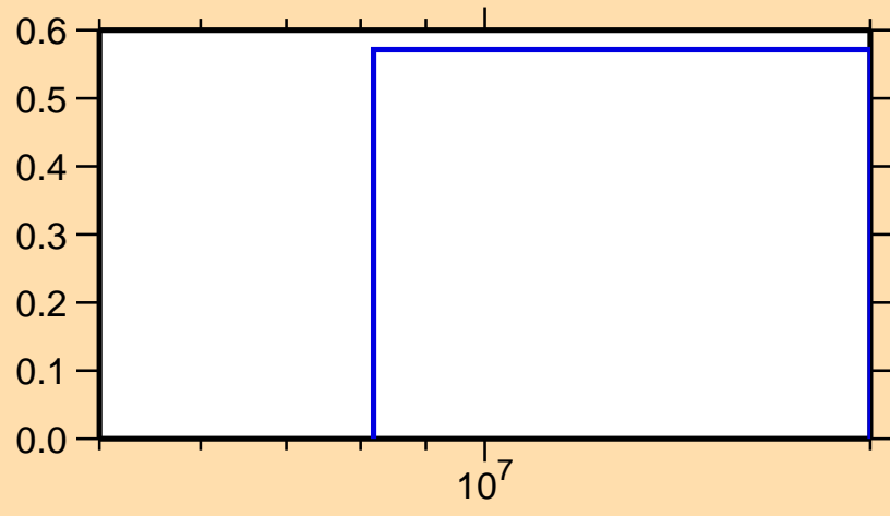
\sigma vs. E for ^{133}\text{Sn}(n,3n)
