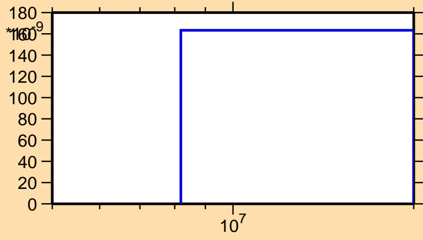
\sigma vs. E for ^{133}\text{Sn}(n,t)
