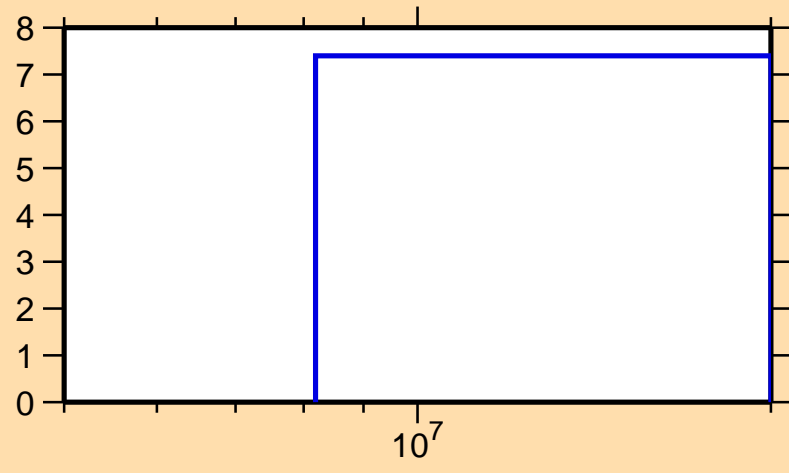
\Delta\sigma/\sigma vs. E for ^{133}\text{Sn}(n,\text{el.})
