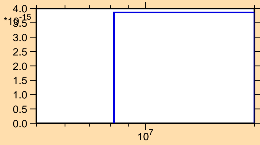
\sigma vs. E for ^{133}\text{Sn}(n,nd)
