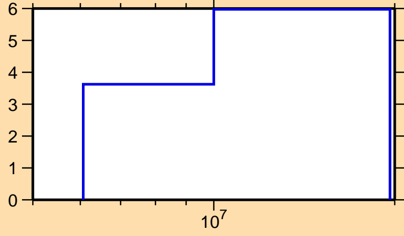
\Delta\sigma/\sigma vs. E for ^{134}\text{Sn}(n,\text{tot.})
