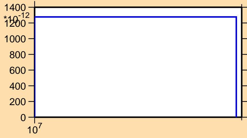
\sigma vs. E for ^{134}\text{Sn}(n,n\alpha)
