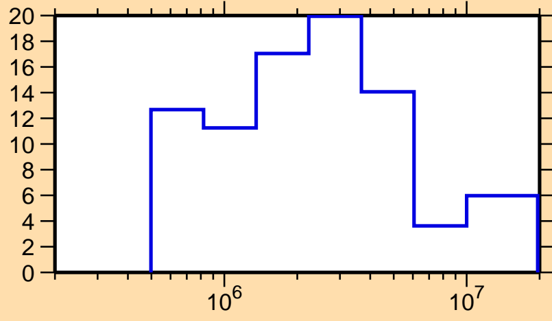
\Delta\sigma/\sigma vs. E for ^{134}\text{Sn}(n,\text{tot.})
