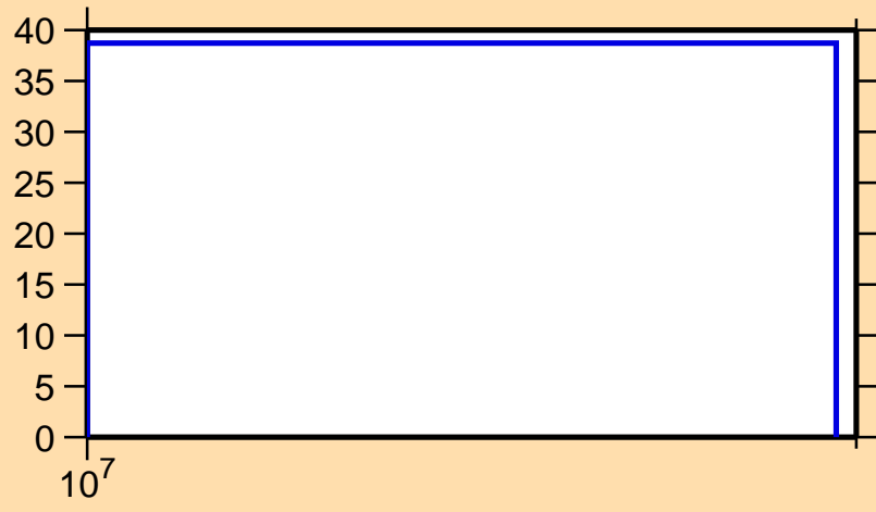
\Delta\sigma/\sigma vs. E for ^{134}\text{Sn}(n,\text{inel.})
