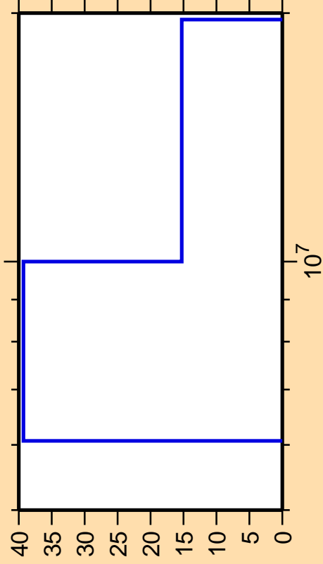
\Delta\sigma/\sigma vs. E for ^{134}\text{Sn}(n,3n)
