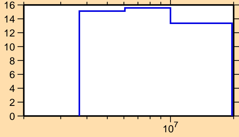
\Delta\sigma/\sigma vs. E for ^{134}\text{Sn}(n,\text{nonel.})
