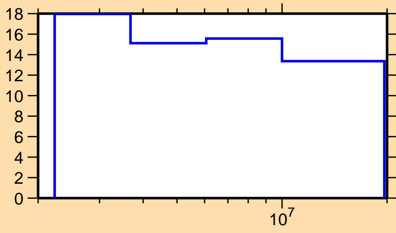
\Delta\sigma/\sigma vs. E for ^{134}\text{Sn}(n,\text{nonel.})
