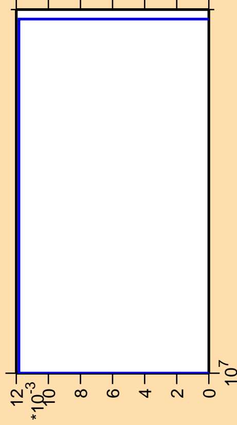
\Delta\sigma/\sigma vs. E for ^{134}\text{Sn}(n,\text{nd})
