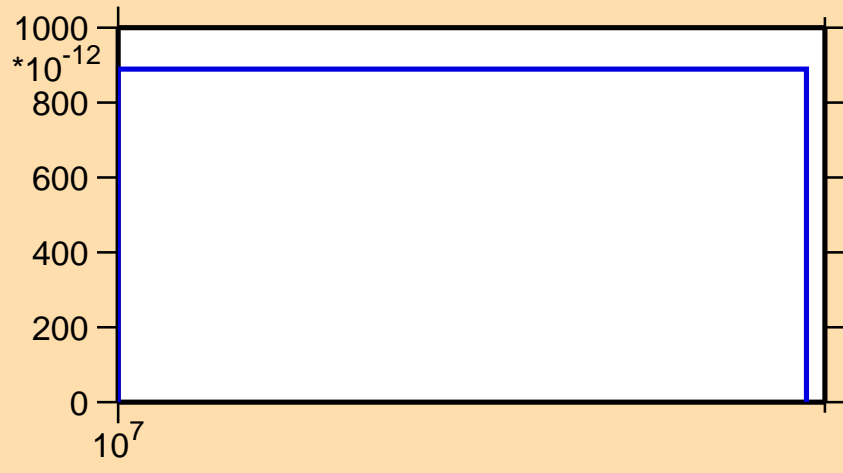
\sigma vs. E for ^{134}\text{Sn}(n,p)
