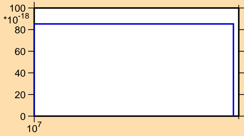
\sigma vs. E for ^{134}\text{Sn}(n,2n\alpha)
