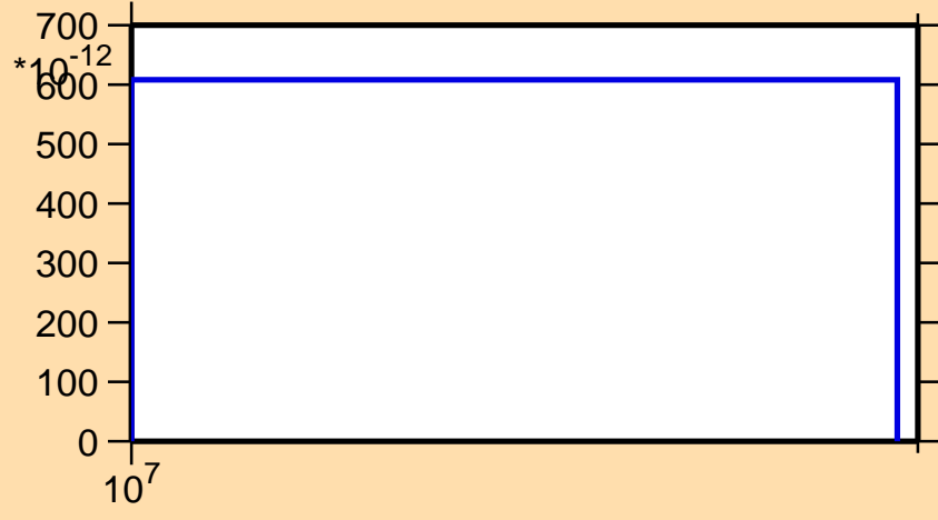
\sigma vs. E for ^{134}\text{Sn}(n,d)
