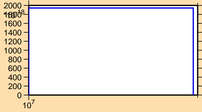
\sigma vs. E for ^{134}\text{Sn}(n,\text{nd})
