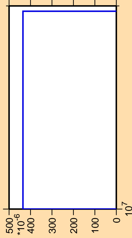
\Delta\sigma/\sigma vs. E for ^{134}\text{Sn}(n,2n\alpha)
