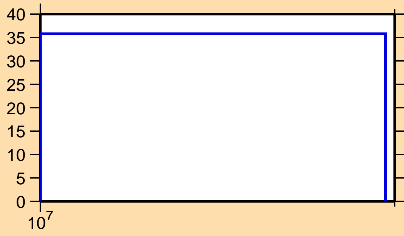
\Delta\sigma/\sigma vs. E for ^{134}\text{Sn}(n,2n)
