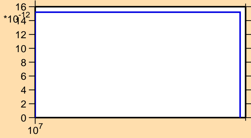
\sigma vs. E for ^{134}\text{Sn}(n,np)
