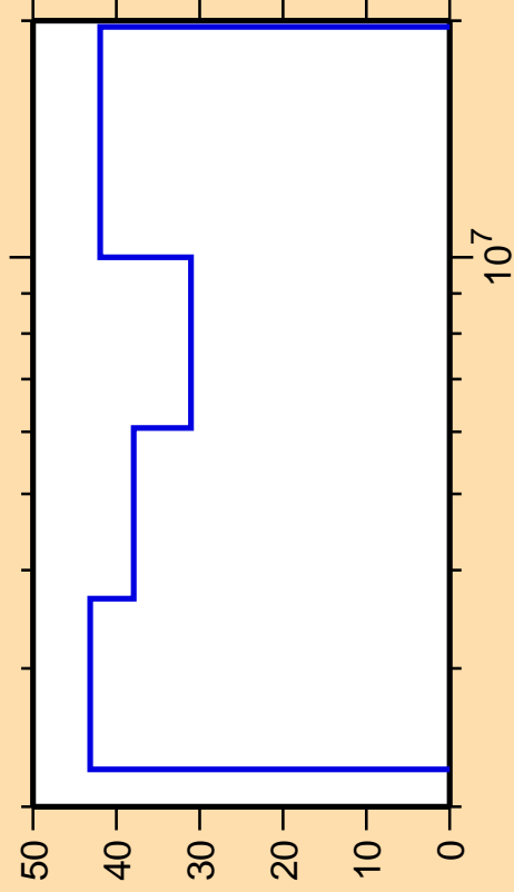
\Delta\sigma/\sigma vs. E for ^{134}\text{Sn}(n,n_4)
