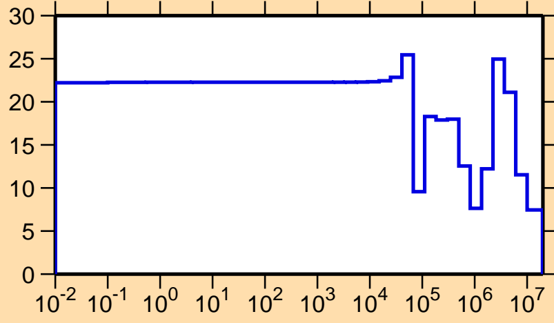
\Delta\sigma/\sigma vs. E for ^{134}\text{Sn}(n,\text{el.})
