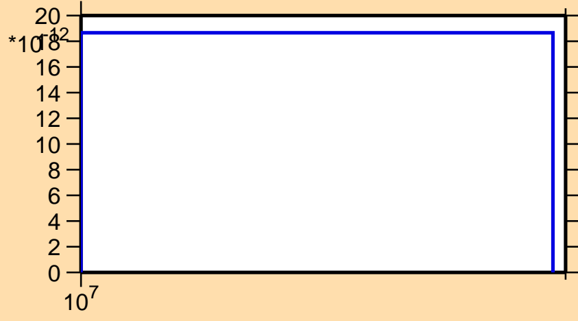
\sigma vs. E for ^{134}\text{Sn}(n,nt)
