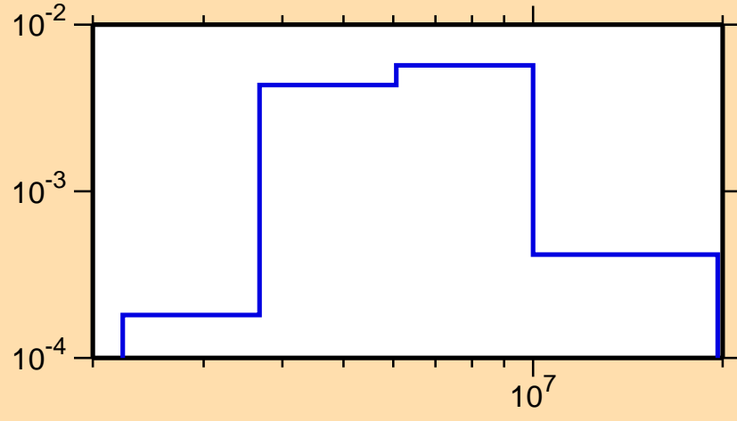
\sigma vs. E for ^{134}\text{Sn}(n,n_4)
