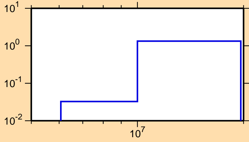
\sigma vs. E for ^{134}\text{Sn}(n,3n)
