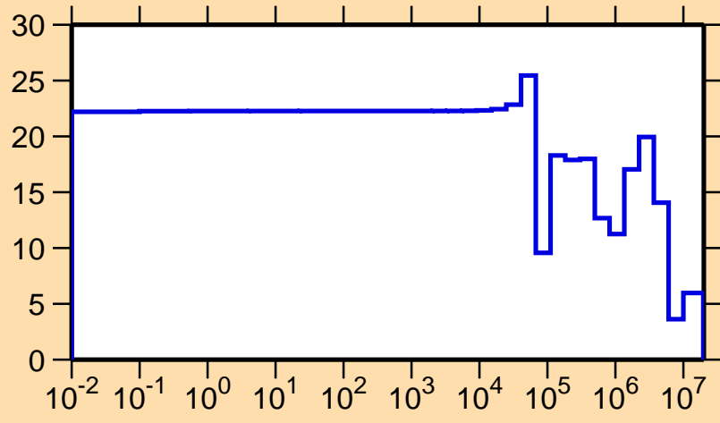
\Delta\sigma/\sigma vs. E for ^{134}\text{Sn}(n,\text{tot.})
