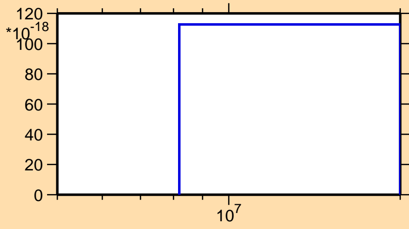
\sigma vs. E for ^{134}\text{Sn}(n,2n\alpha)
