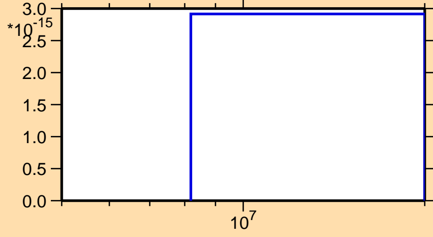
\sigma vs. E for ^{134}\text{Sn}(n,nd)
