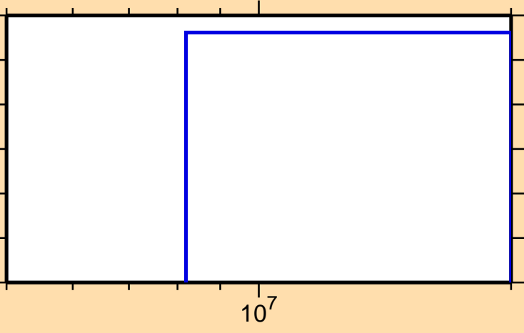
\sigma vs. E for ^{134}\text{Sn}(n,\alpha)
