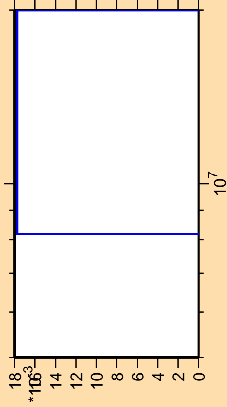
\Delta\sigma/\sigma vs. E for ^{134}\text{Sn}(n,nd)
