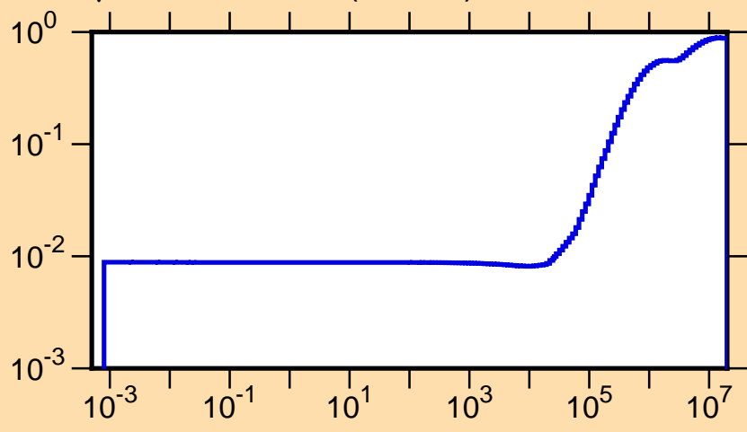
\mu vs. E for ^{76}\text{Sr}(\text{mt251})
